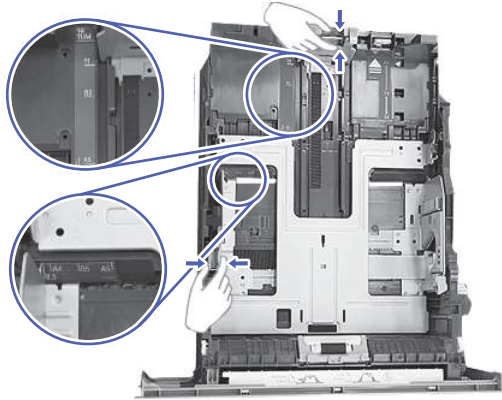
Figure 9-15 Adjust guides
