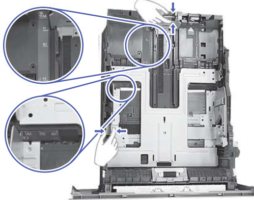
Figure 9-17 Adjust guides
