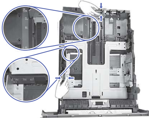
Figure 9-18 Adjust guides
