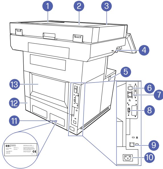
Figure 1-9 Printer back view:5602, 5602dn, 5602f, 5602zfw
