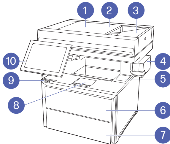
Figure 1-7 Printer front view - 5602f
