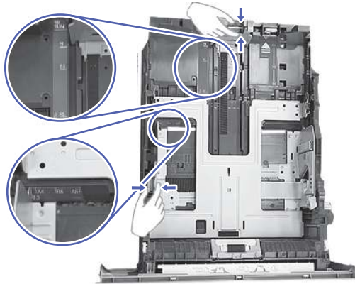
Figure 9-19 Adjust guides
