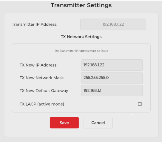
FIGURE 7-26: NETWORK SETTINGS OPTIONS
