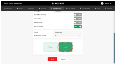
FIGURE 7-58: MOUSE SECTOR EXAMPLE
