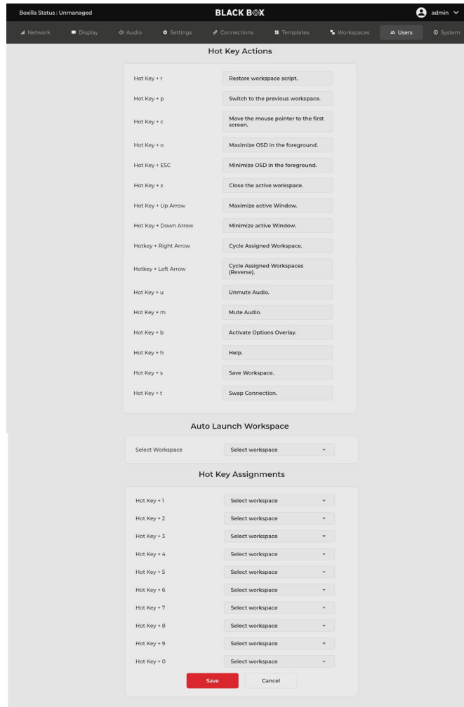
FIGURE 7-97: USER WORKSPACE AND HOT KEY SELECTION SCREEN
