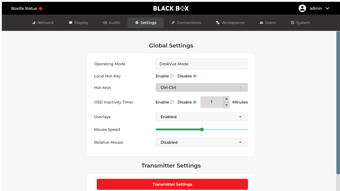
FIGURE 7-19: GLOBAL SETTINGS PAGE
