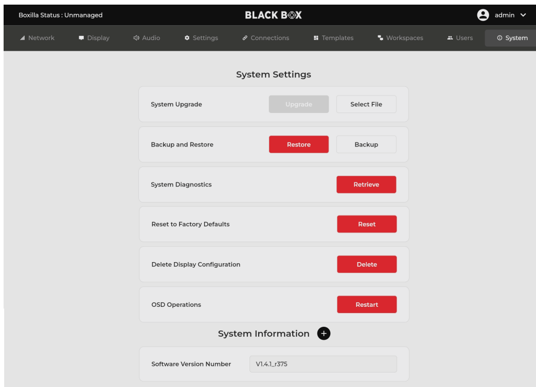
FIGURE 7-98: SYSTEM SETTINGS SCREEN
