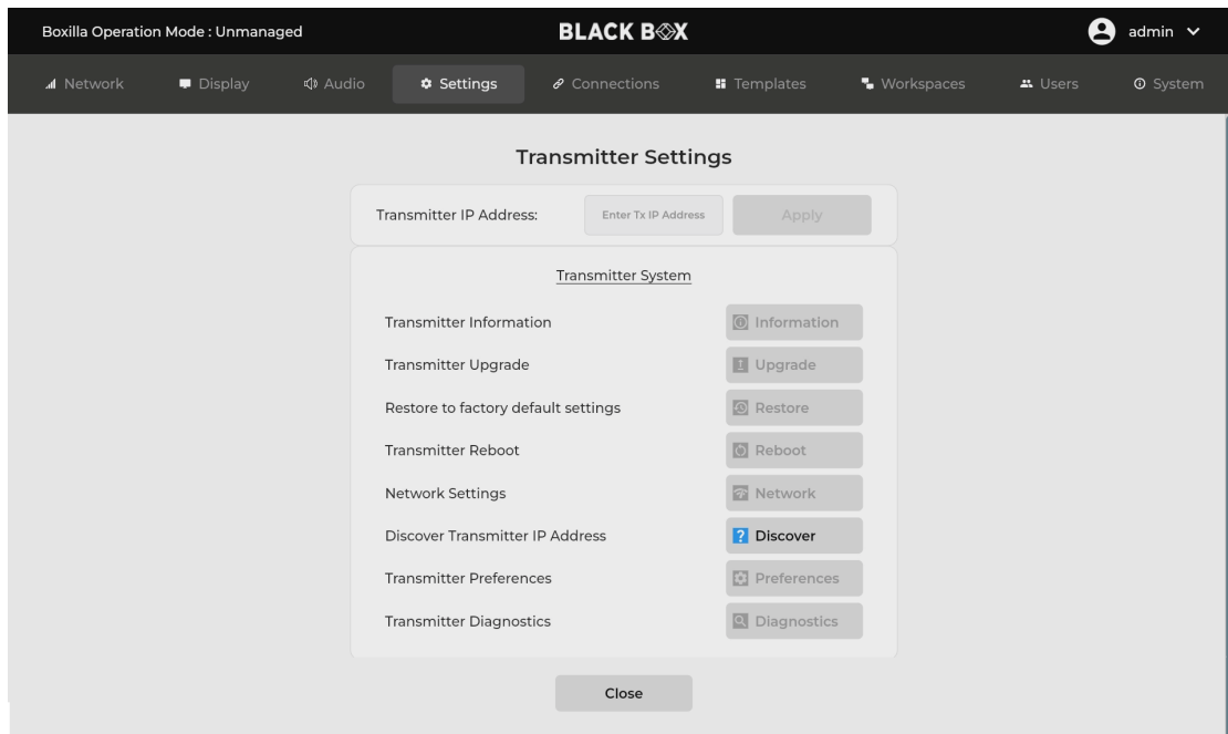
FIGURE 7-21: TRANSMITTER SETTINGS PAGE
