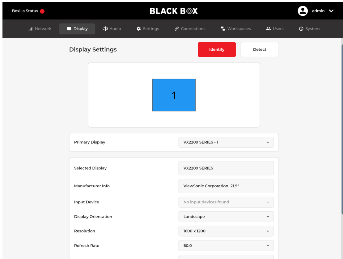
FIGURE 7-13: DISPLAY SETTINGS SCREEN
