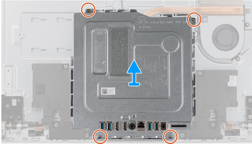
Figure 26. Removing the system-board shield
