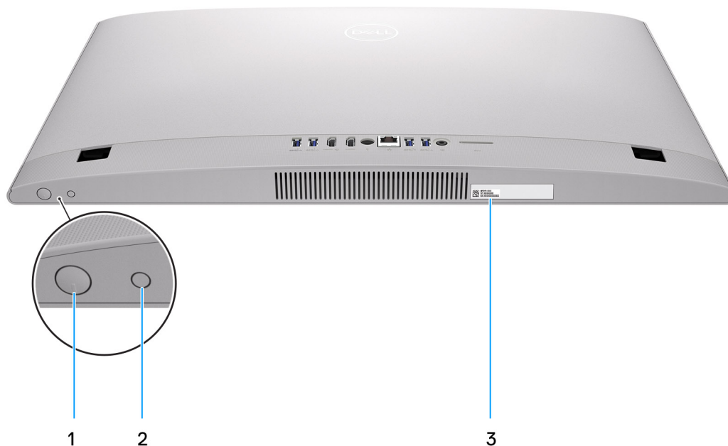
Figure 5. Bottom view
