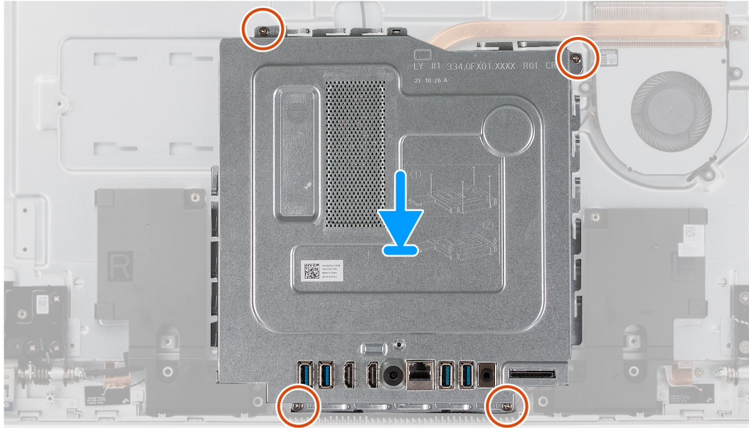
Figure 27. Installing the system-board shield
