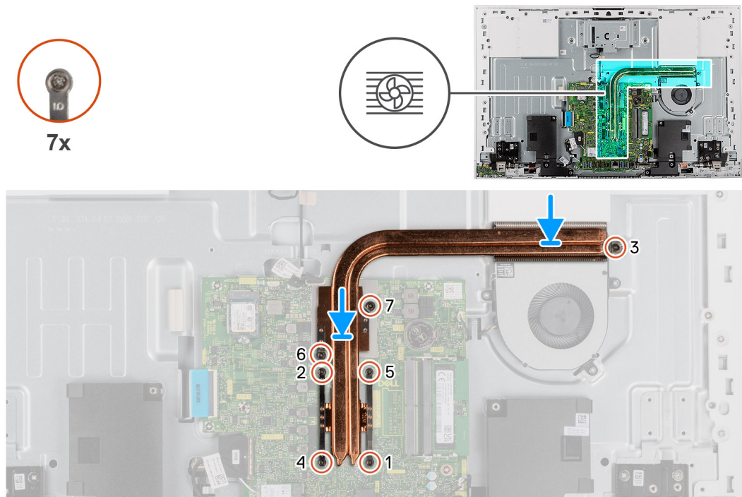
Figure 45. Installing the heat sink- discrete
