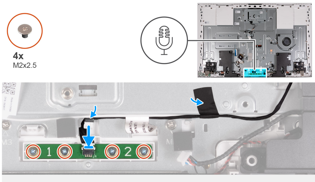
Figure 57. Installing the microphone module
