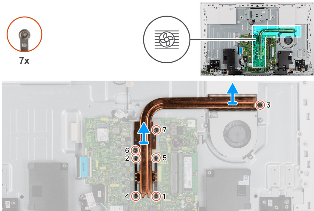
Figure 44. Removing the heat sink- discrete
