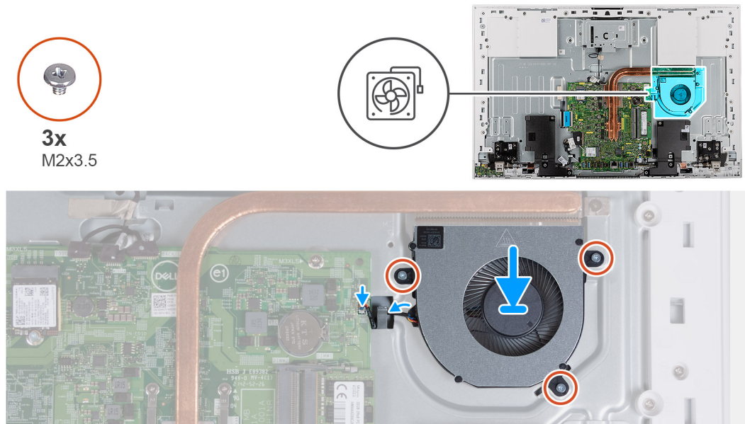
Figure 37. Installing the fan
