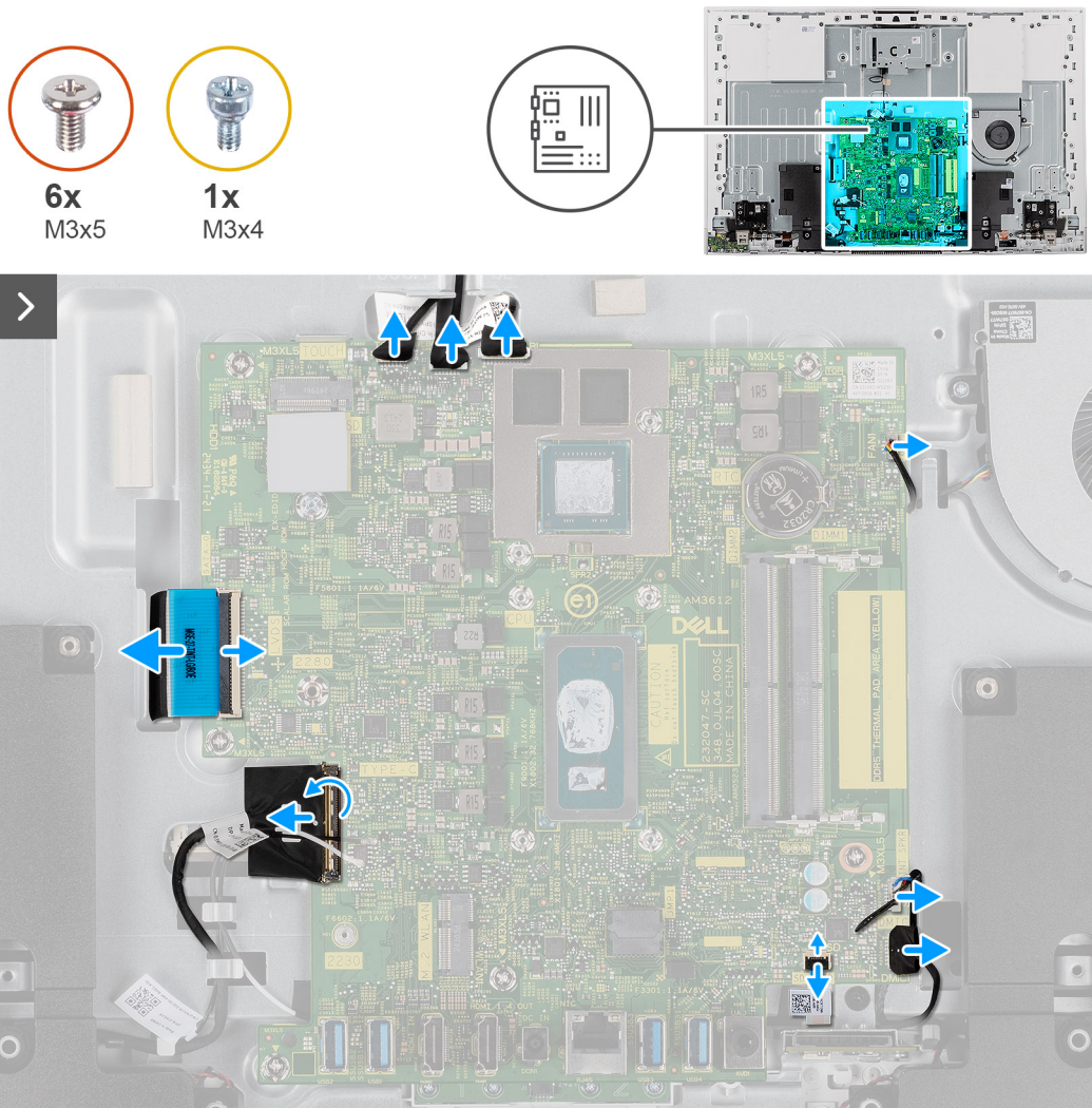
Figure 51. Removing the system board
