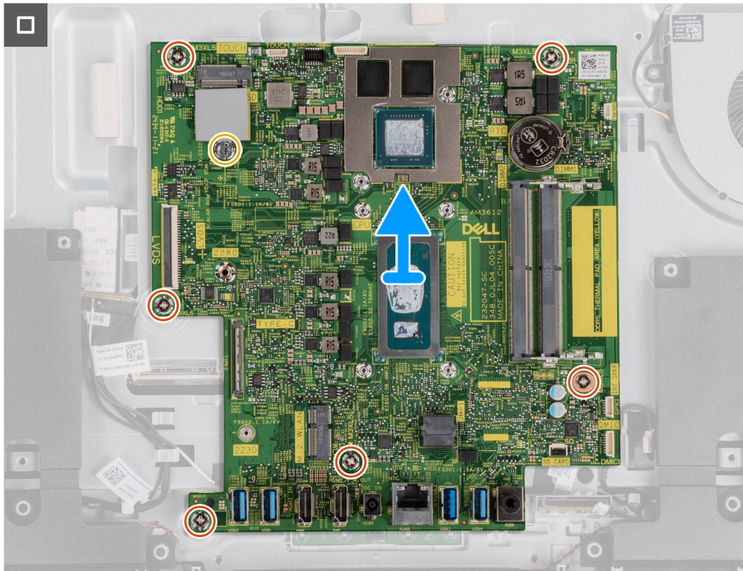
Figure 52. Lifting the system board off the chassis
