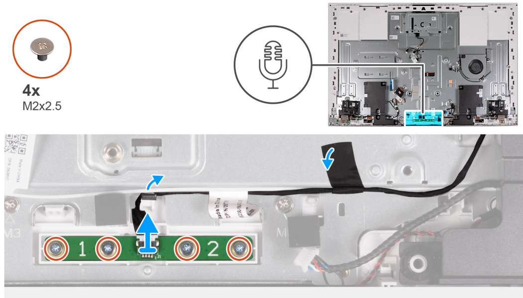
Figure 56. Removing the microphone module
