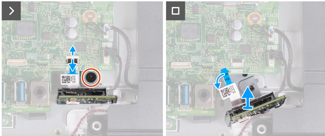
Figure 46. Removing the media-card reader
