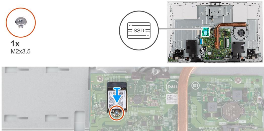
Figure 28. Removing the M.2 2230 solid-state drive
