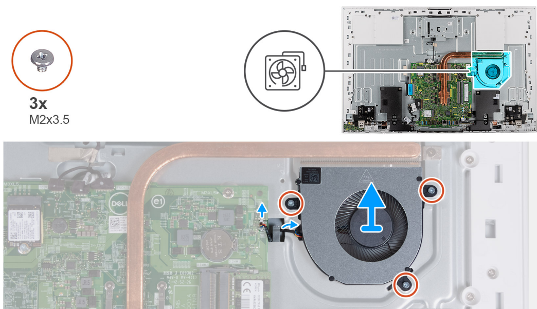
Figure 36. Removing the fan
