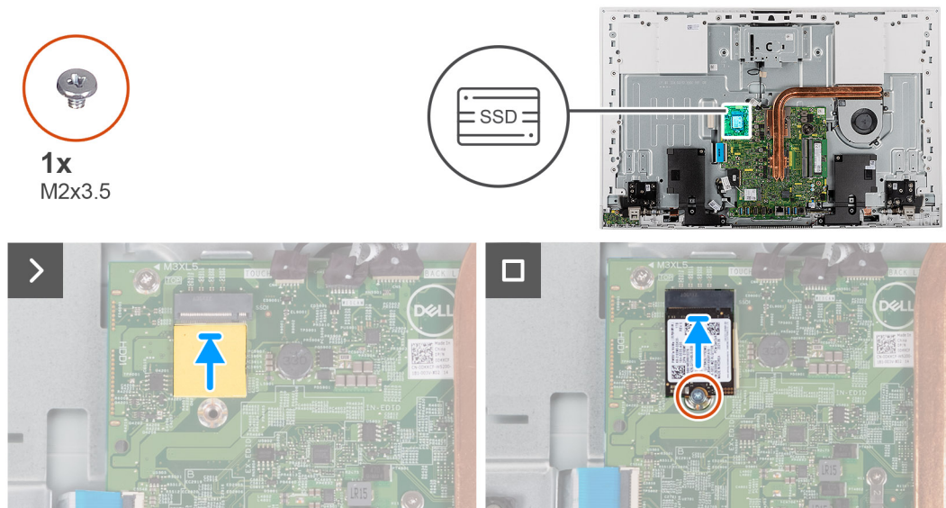
Figure 29. Installing the M.2 2230 solid-state drive
