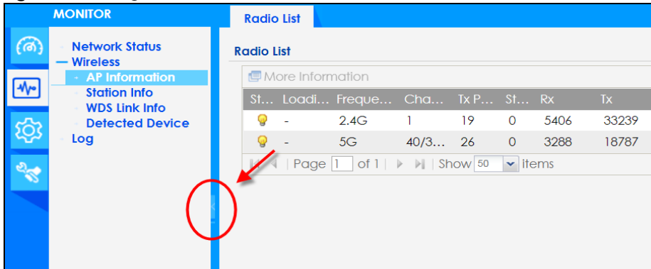
Figure 36 Navigation Panel
