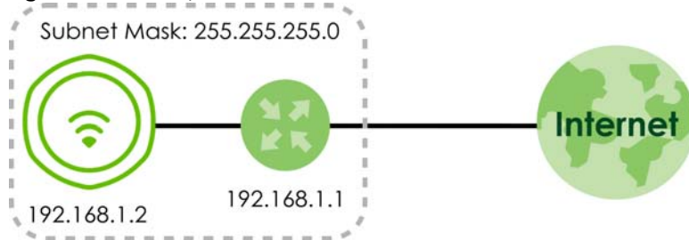
Figure 70 IP Setup
