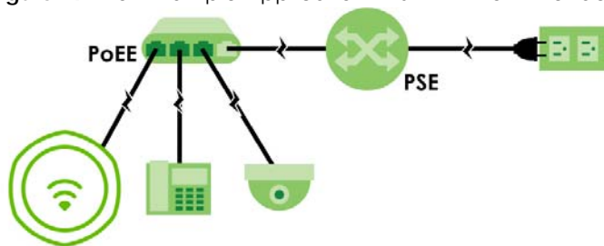
Figure 29 PoE Example Application - PSE with PoE Extender
