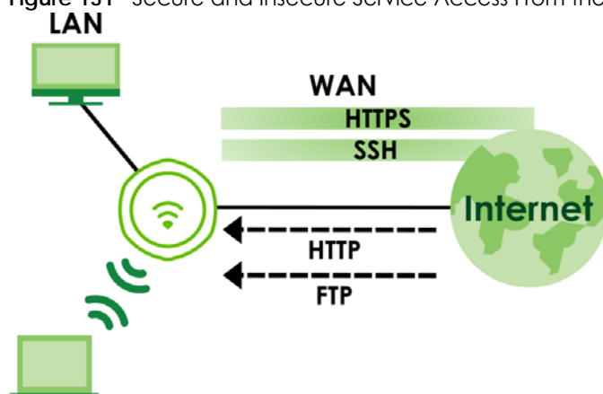
Figure 131 Secure and Insecure Service Access From the WAN
