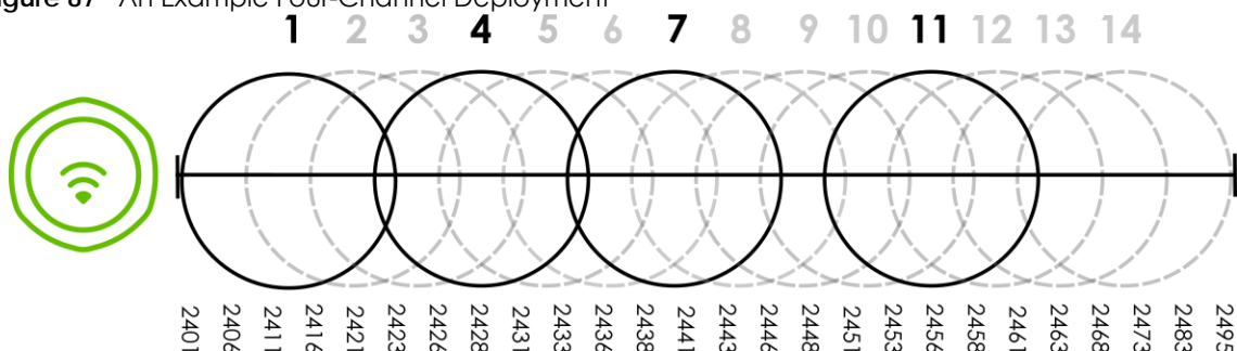
Figure 87 An Example Four-Channel Deployment
