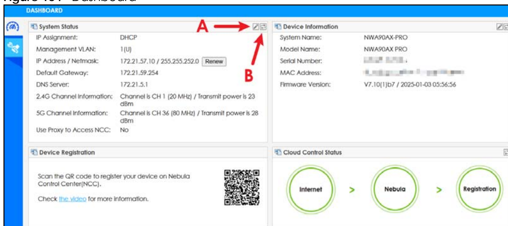
Figure 164 Dashboard
