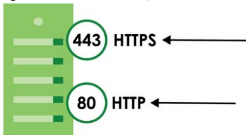
Figure 132 HTTP/HTTPS Implementation
