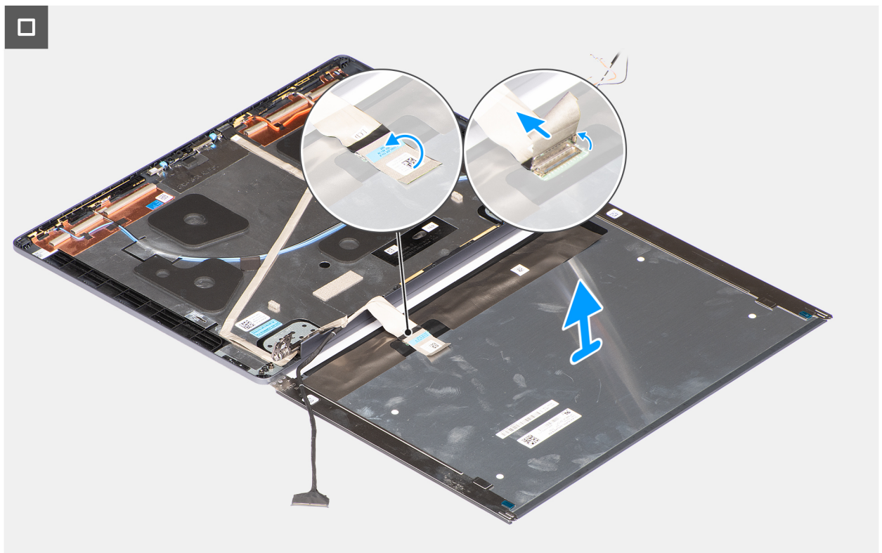
Figure 70. Removing the display panel
