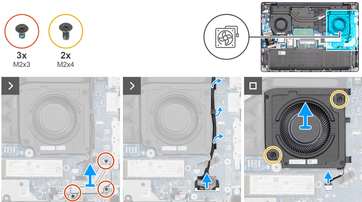
Figure 38. Removing the left/video fan
