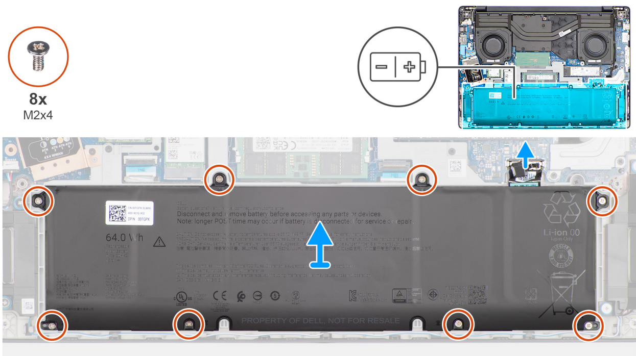
Figure 17. Removing the battery
