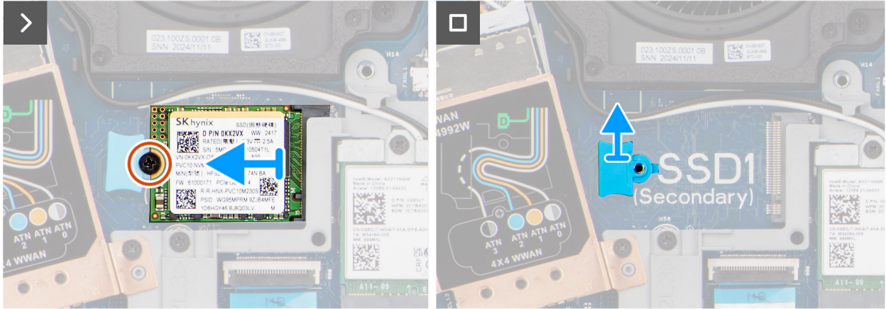
Figure 23. Removing the M.2 2230 solid state drive
