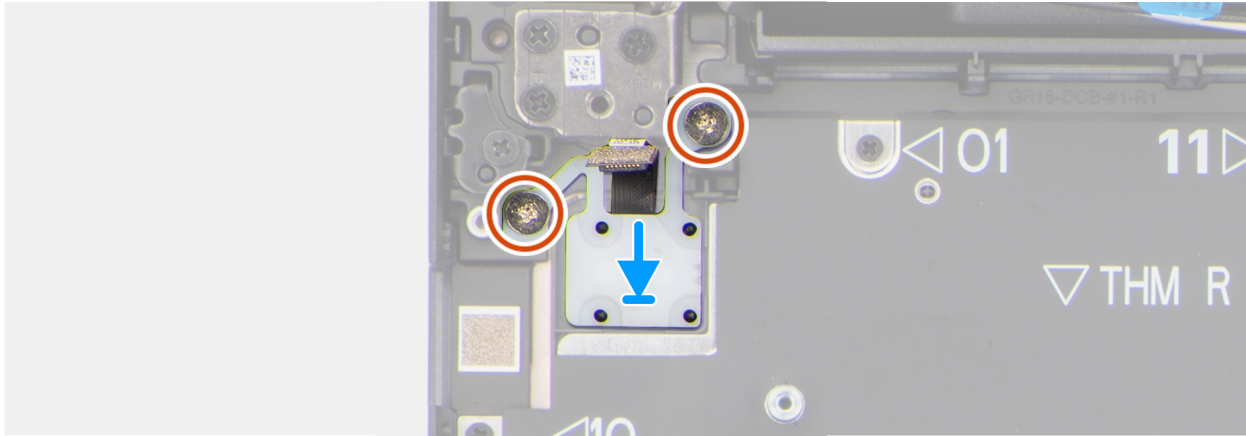
Figure 97. Installing the power button
