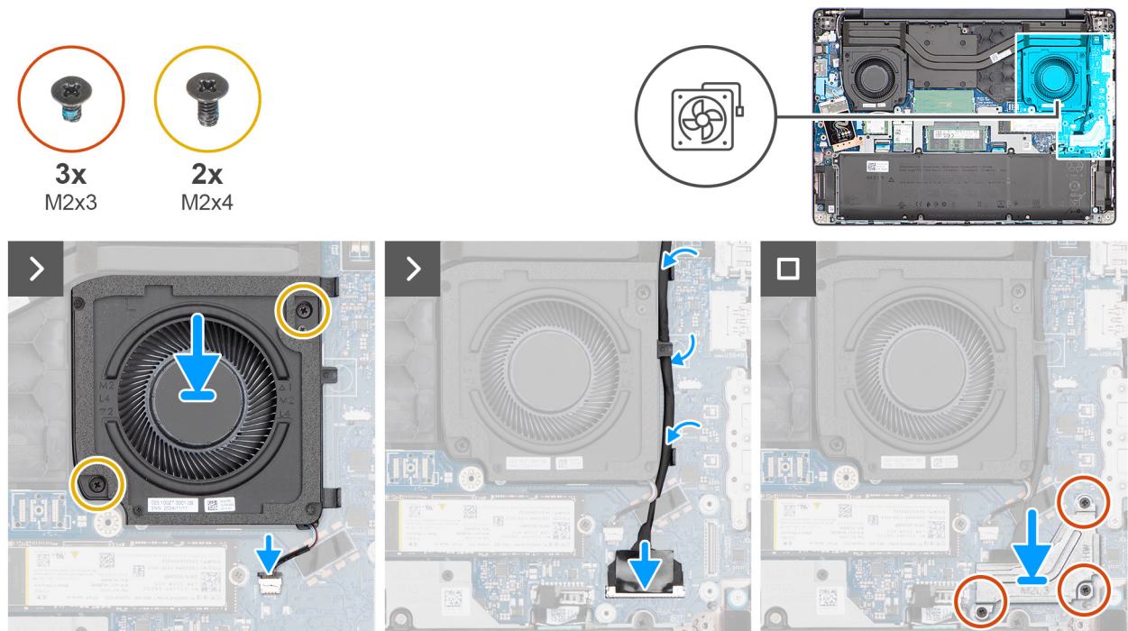
Figure 39. Installing the left/video fan
