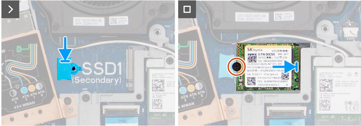
Figure 24. Installing the M.2 2230 solid state drive
