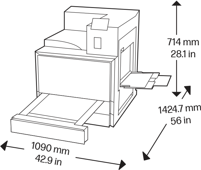
Figure 1-10 Printer dimensions (dn model) fully open
