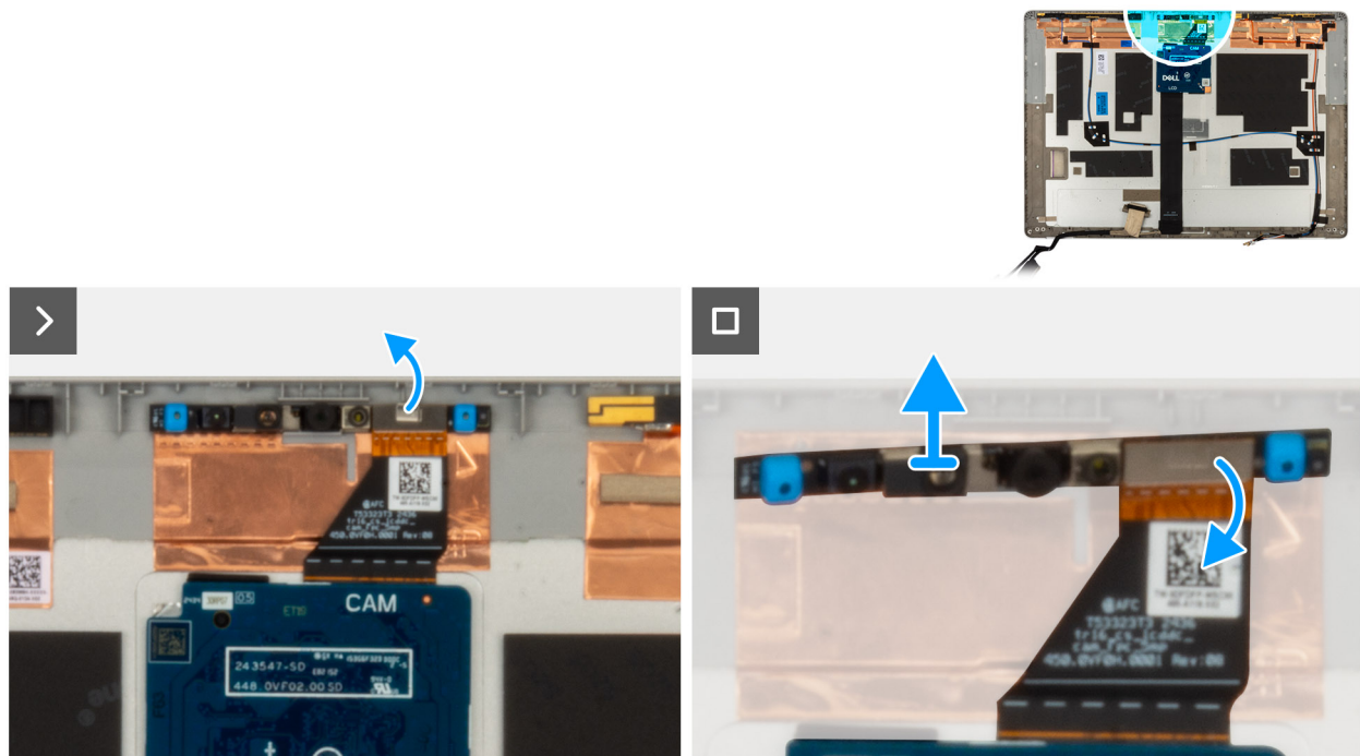
Figure 68. Removing the camera module
