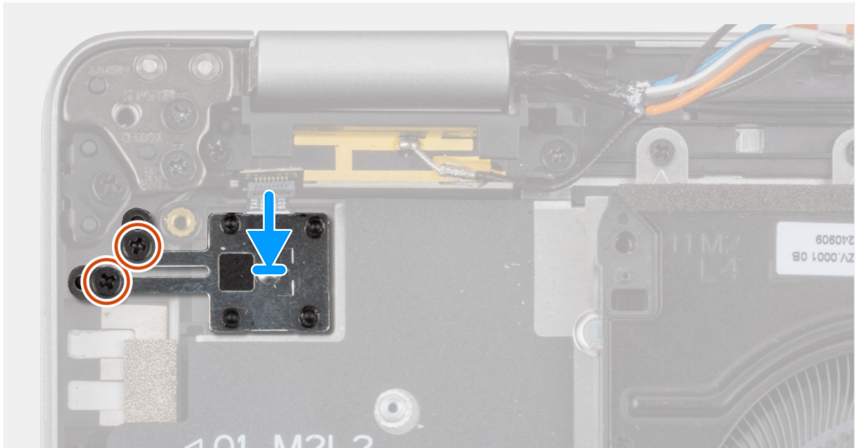
Figure 48. Installing the power button with optional fingerprint reader
