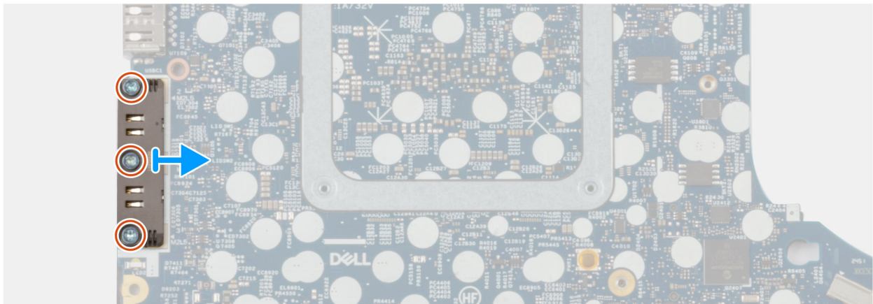
Figure 49. Removing the USB Type-C Connector Module
