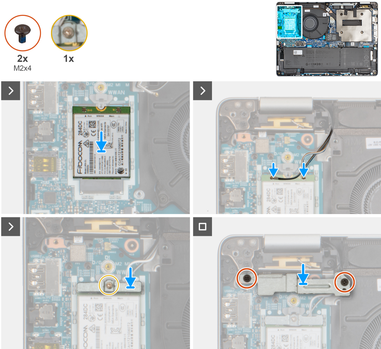
Figure 24. Installing the 4G WWAN card
