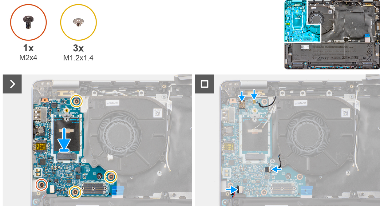
Figure 46. Installing the I/O board
