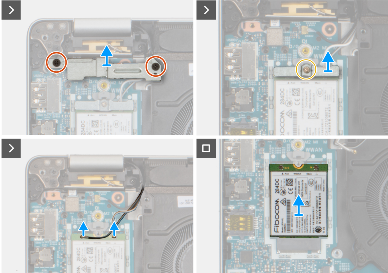
Figure 23. Removing the 4G WWAN card
