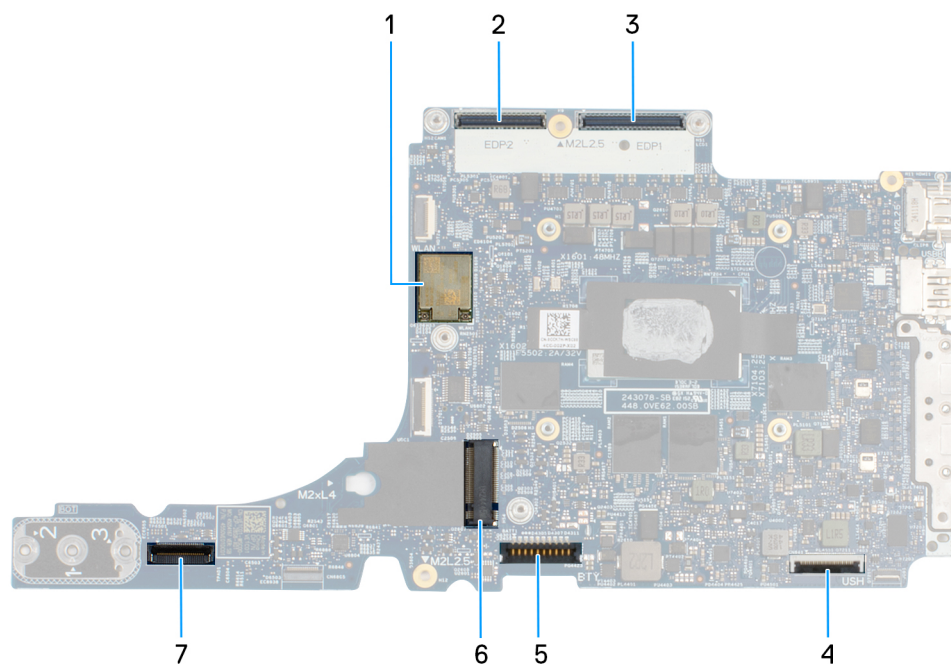
Figure 39. System board connectors
