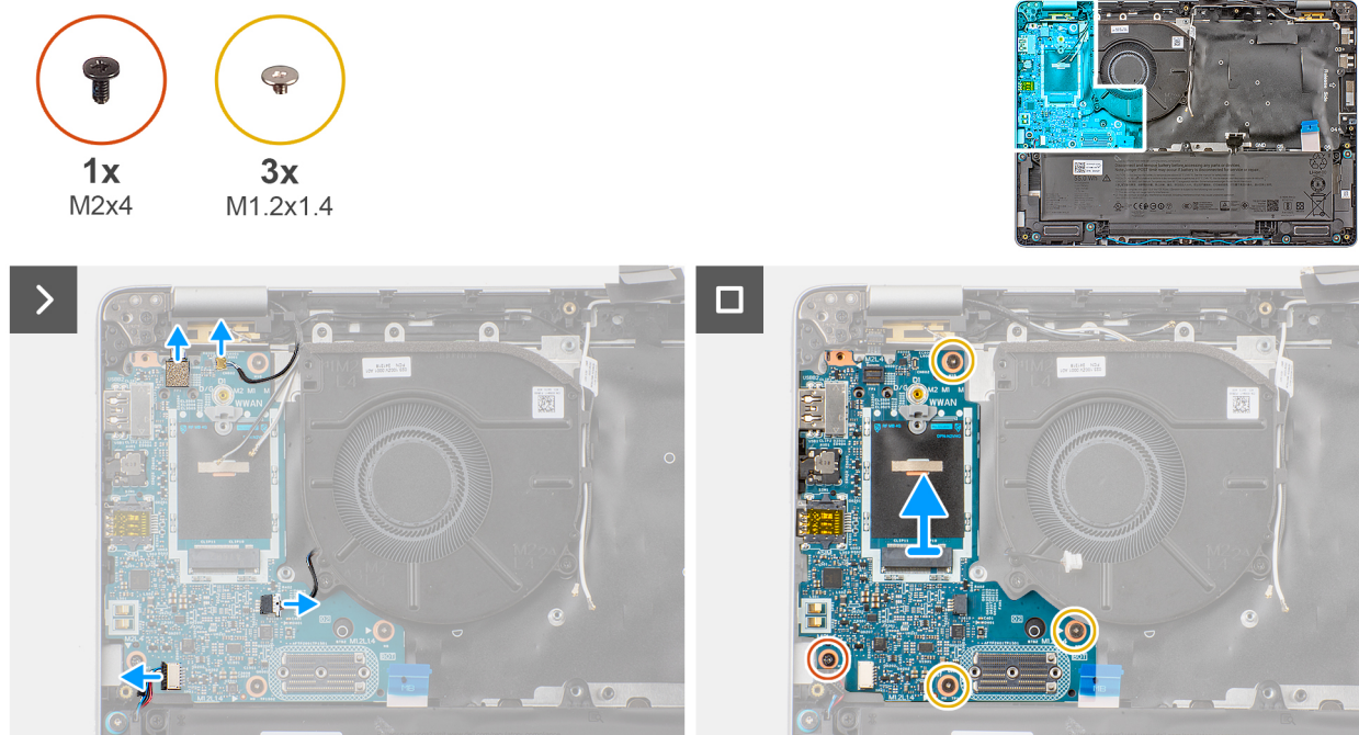
Figure 45. Removing the I/O board
