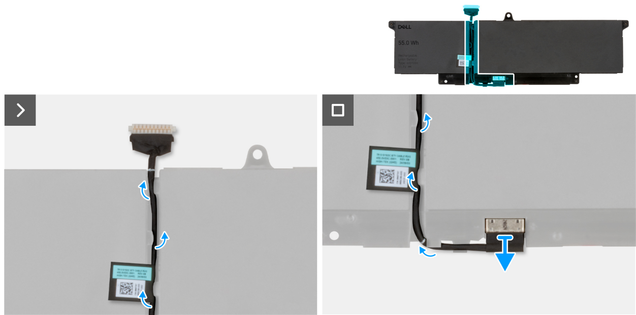
Figure 21. Removing battery cable
