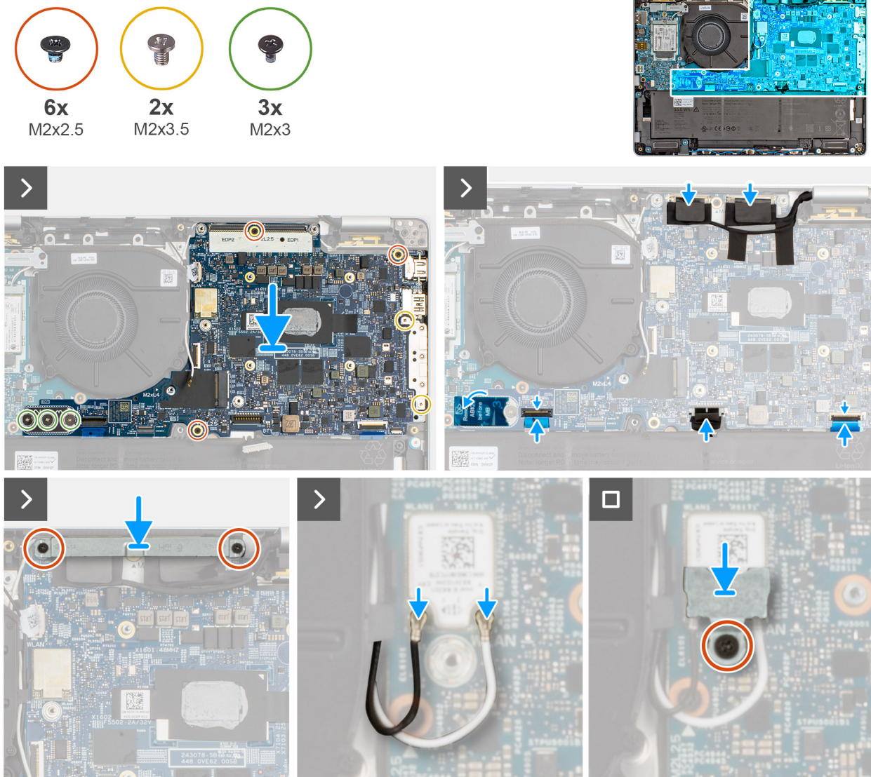
Figure 40. Installing the system board
