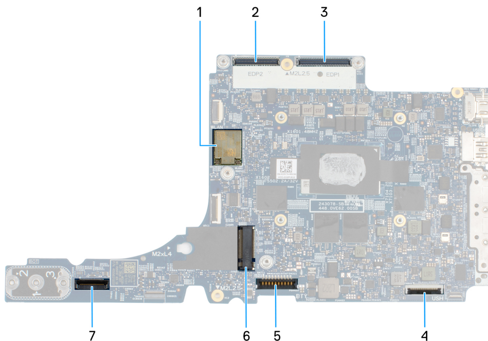
Figure 37. System board connectors
