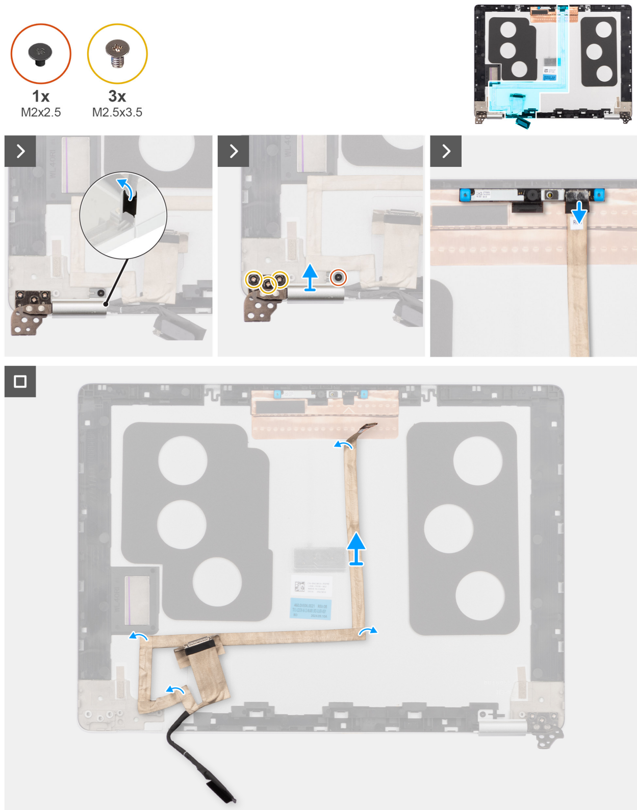
Figure 70. Removing the display cable
