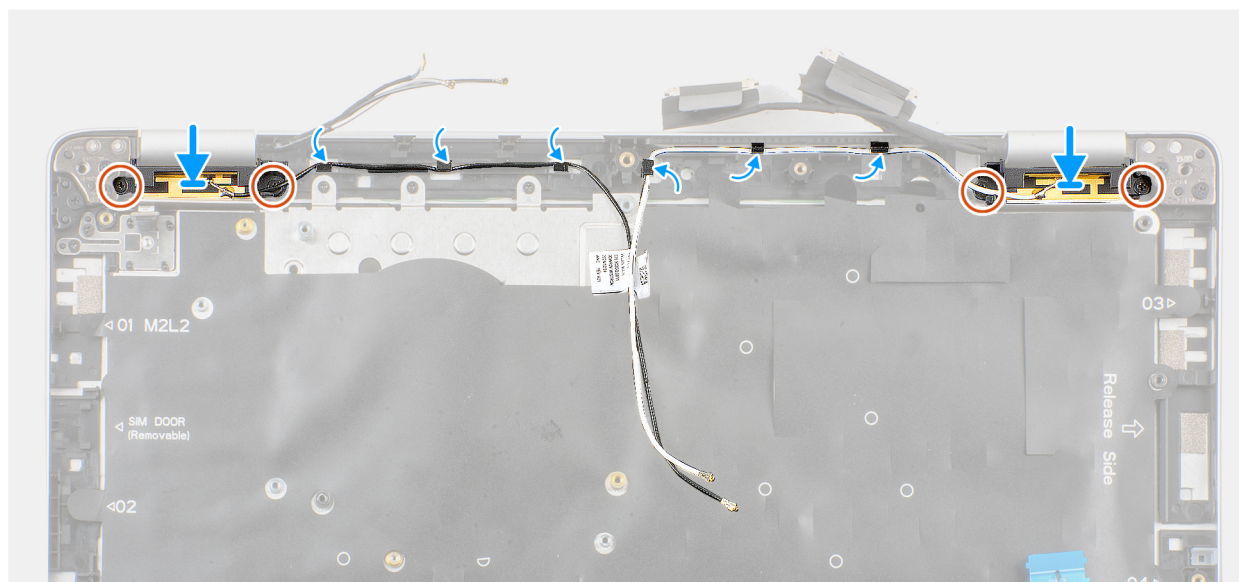
Figure 42. Installing the WLAN antenna module
