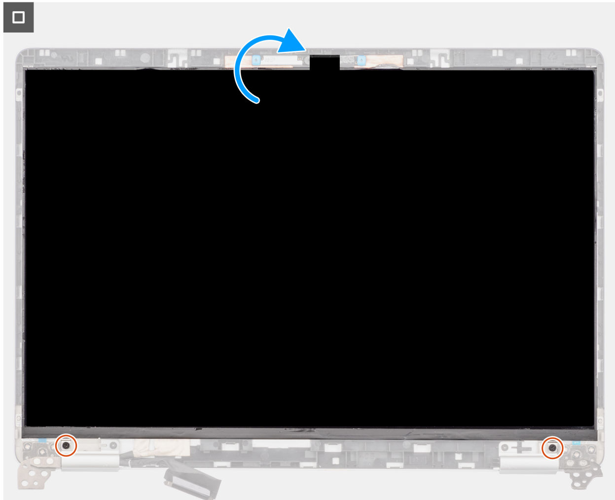
Figure 65. Installing the display panel
