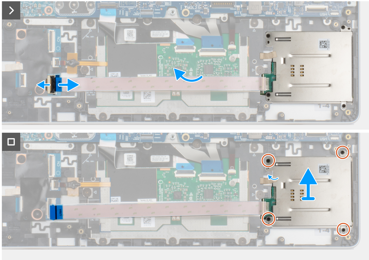
Figure 35. Removing the smart-card reader
