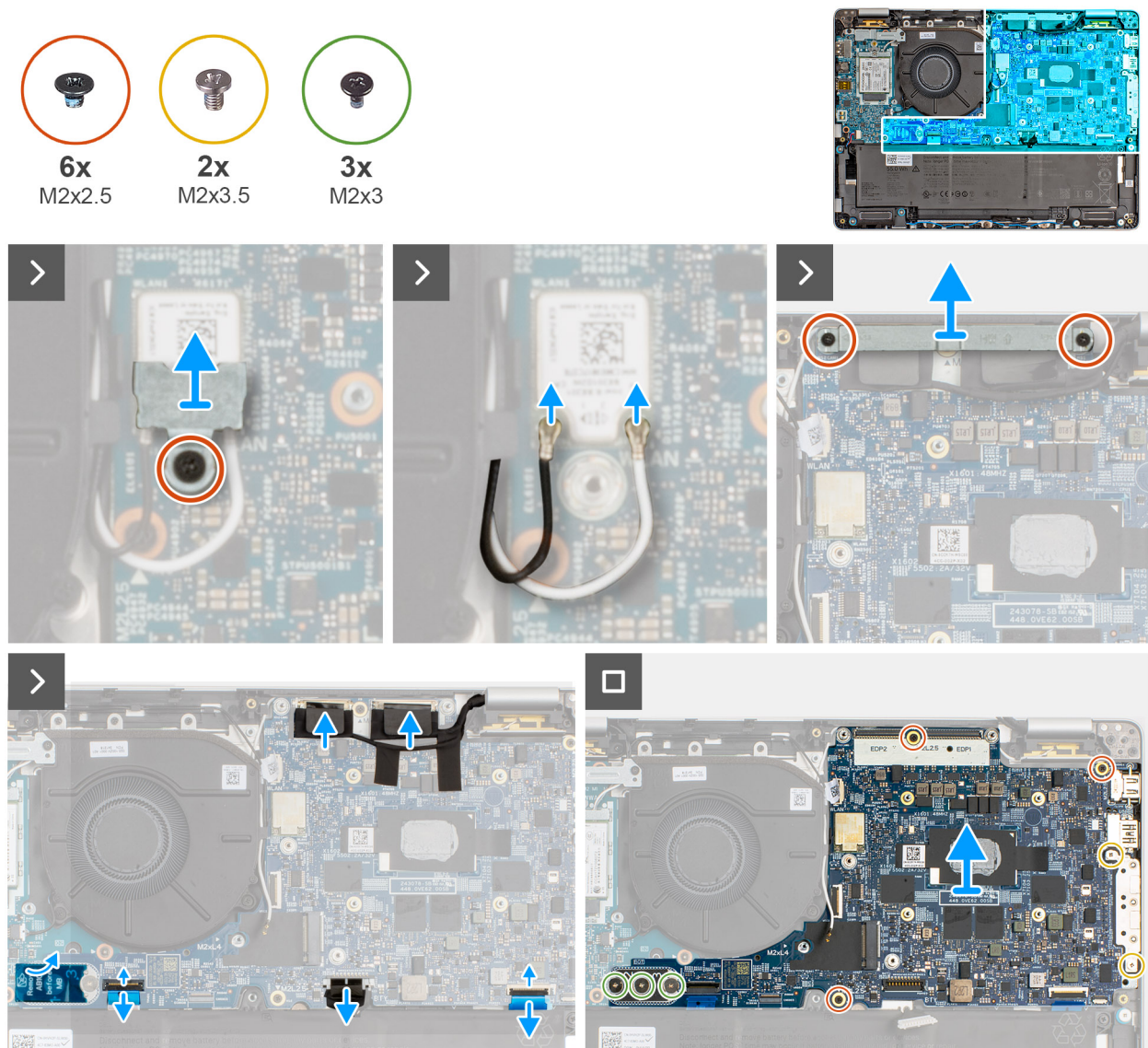
Figure 38. Removing the system board
