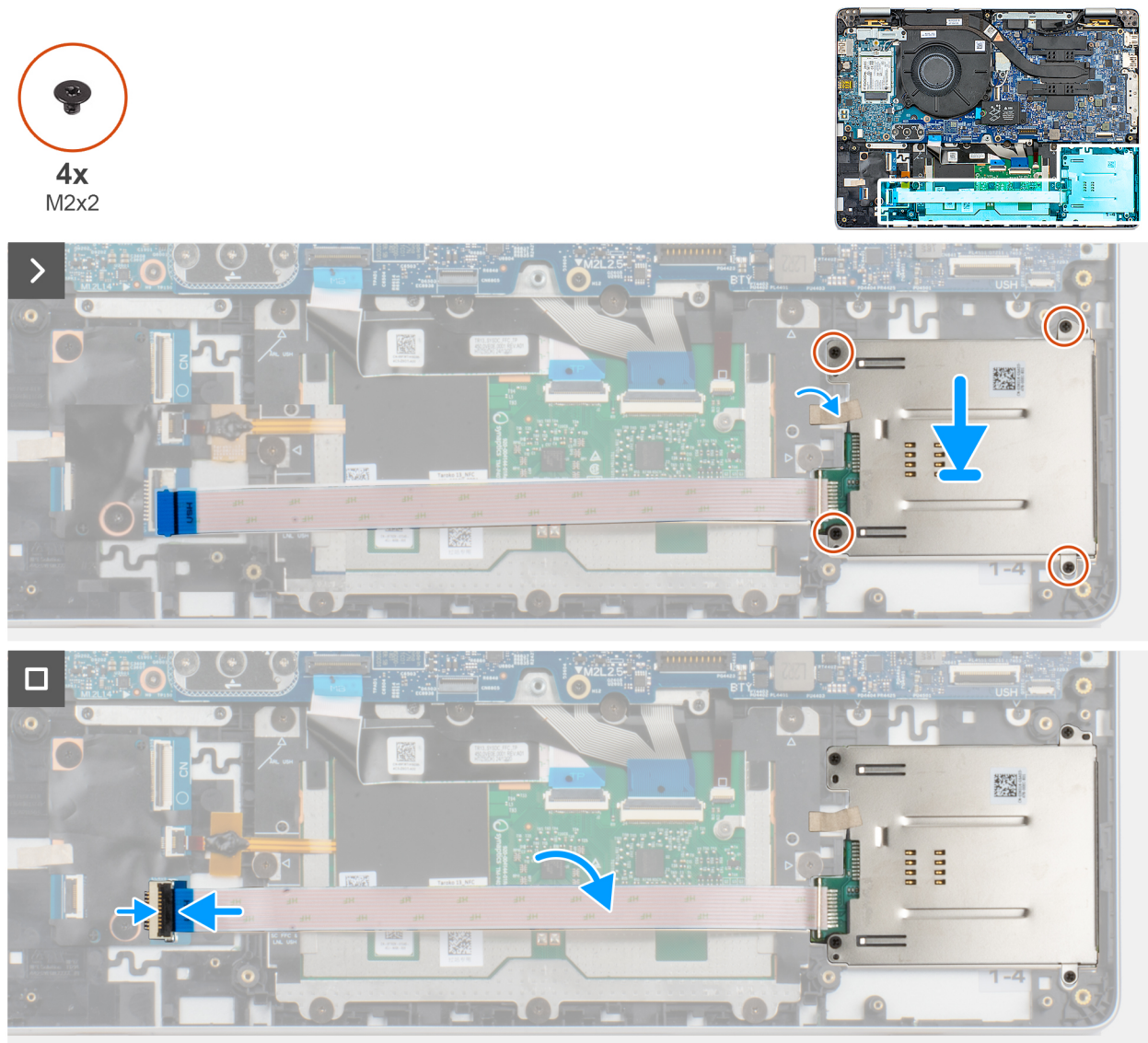
Figure 36. Installing the smart-card reader
