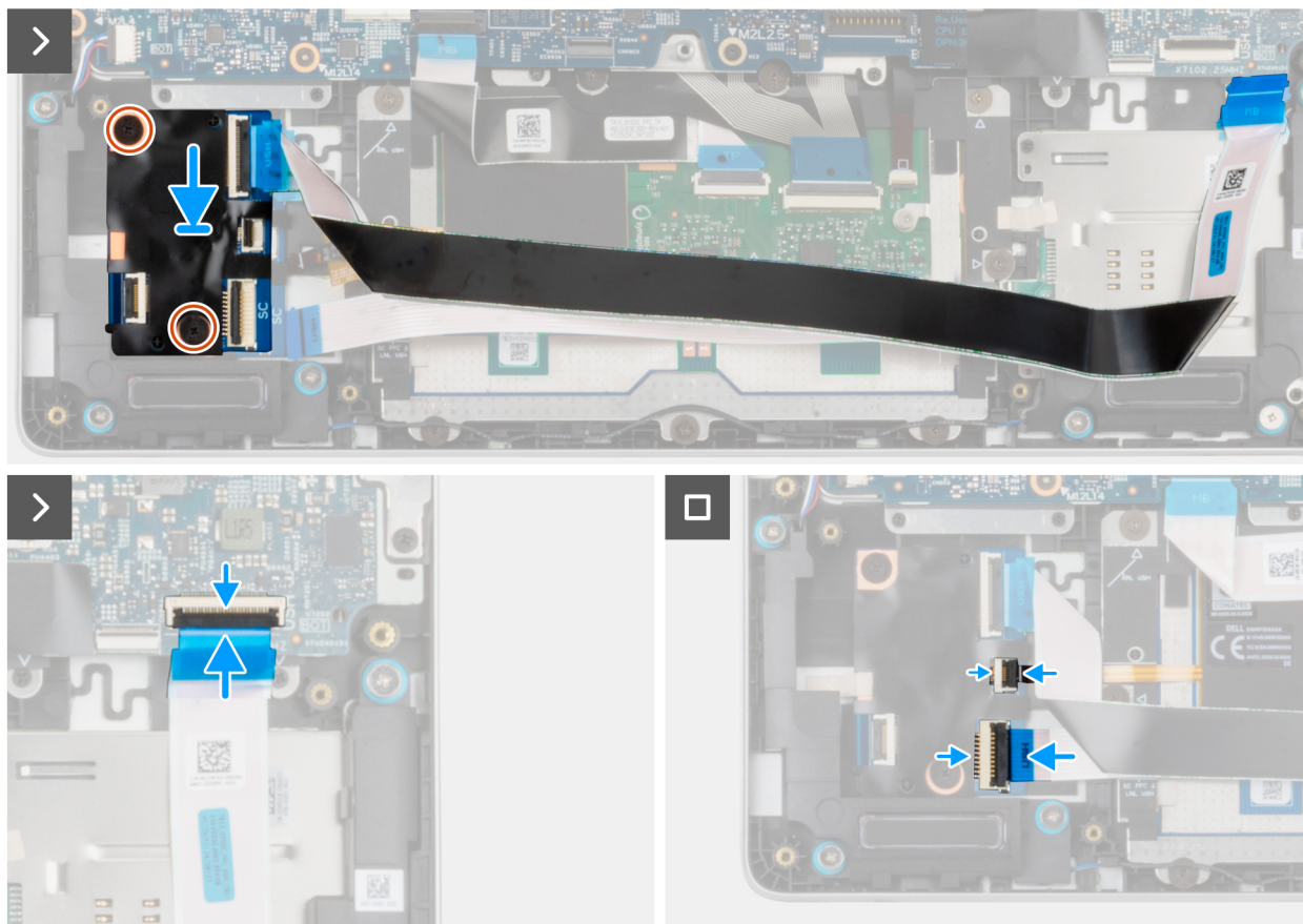
Figure 34. Installing the USH daughterboard
