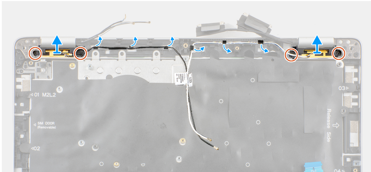
Figure 41. Removing the WLAN antenna module
