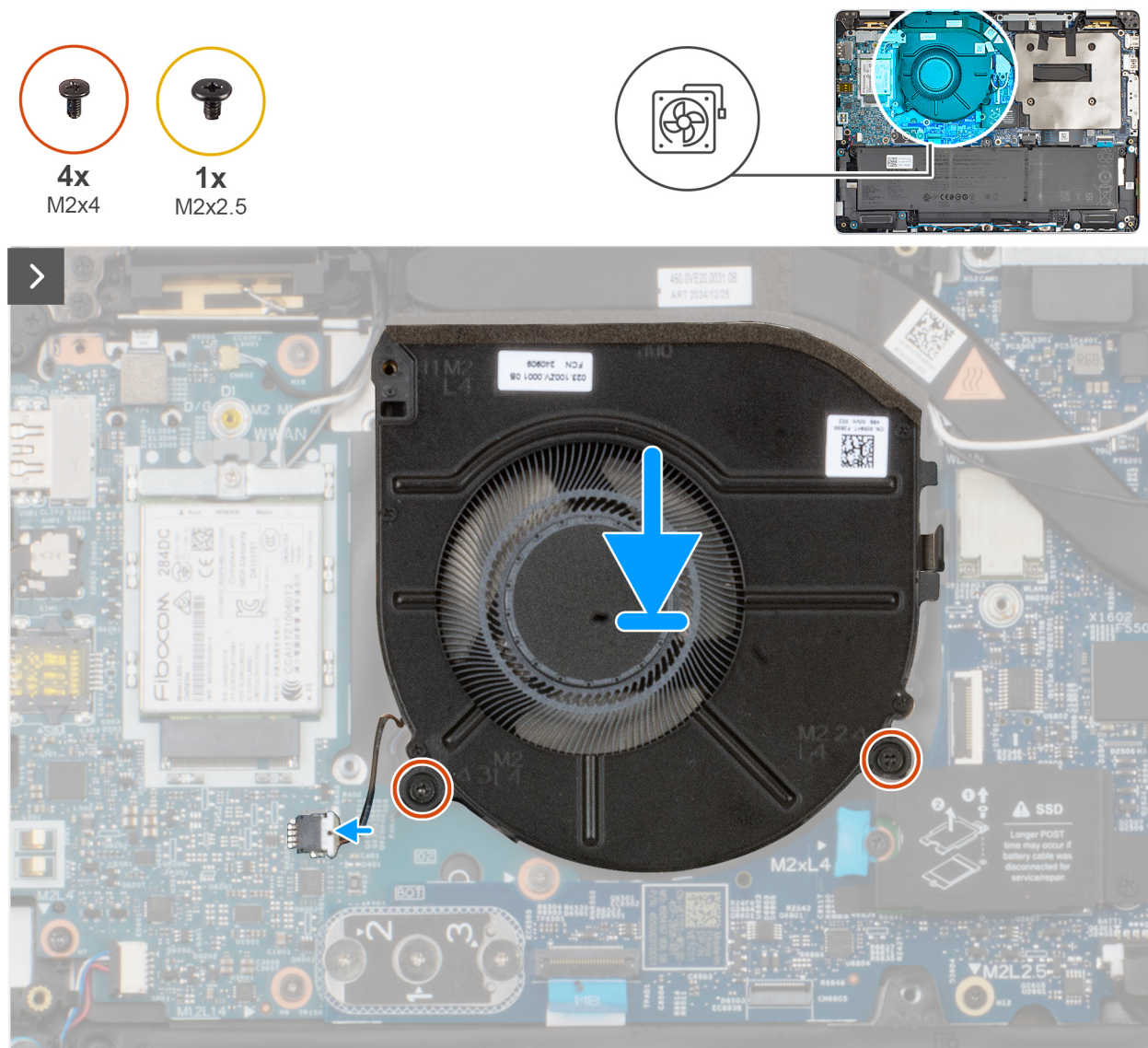
Figure 31. Installing the fan
