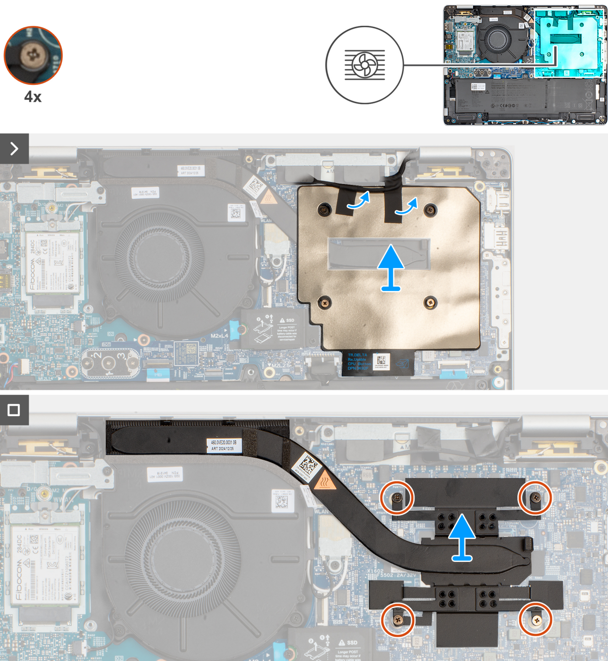
Figure 43. Removing the heat sink
