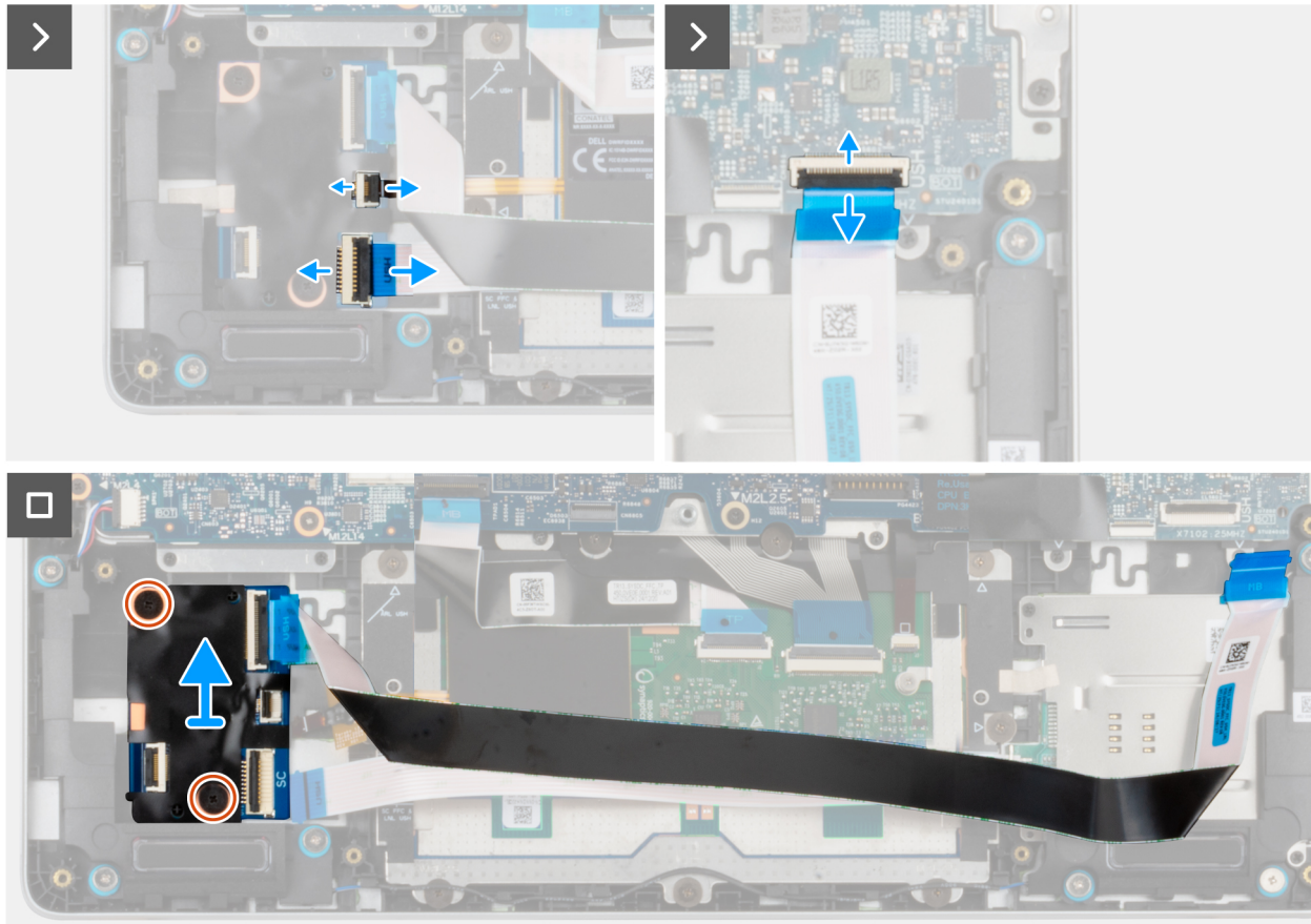
Figure 33. Removing the USH daughterboard
