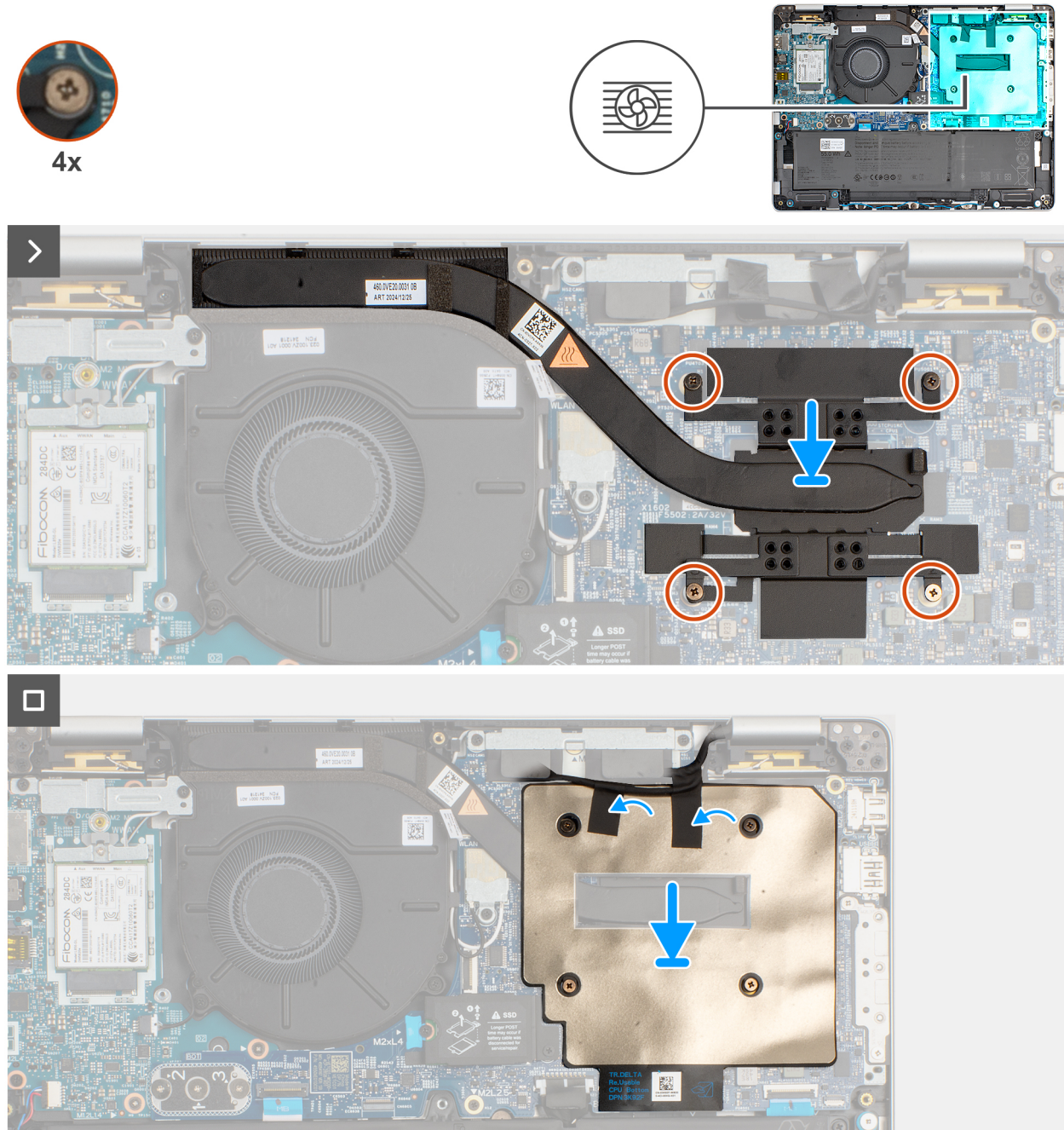
Figure 44. Installing the heat sink
