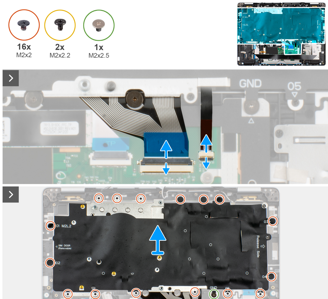
Figure 51. Removing the keyboard
