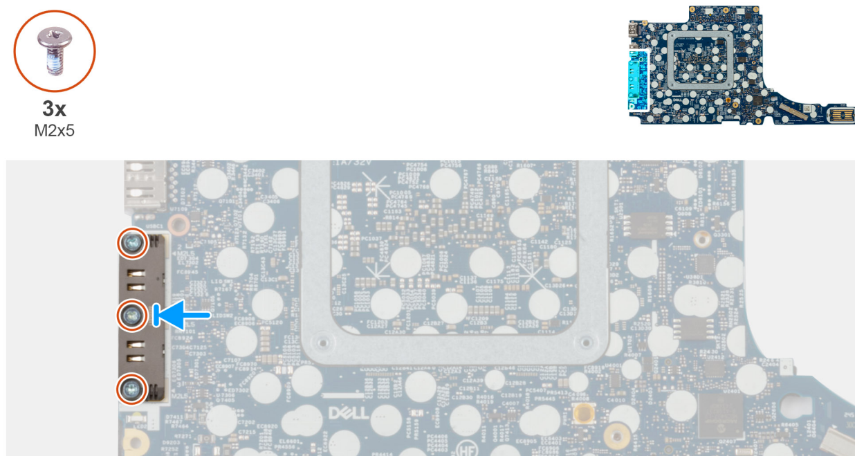
Figure 50. Installing the USB Type-C connector module
