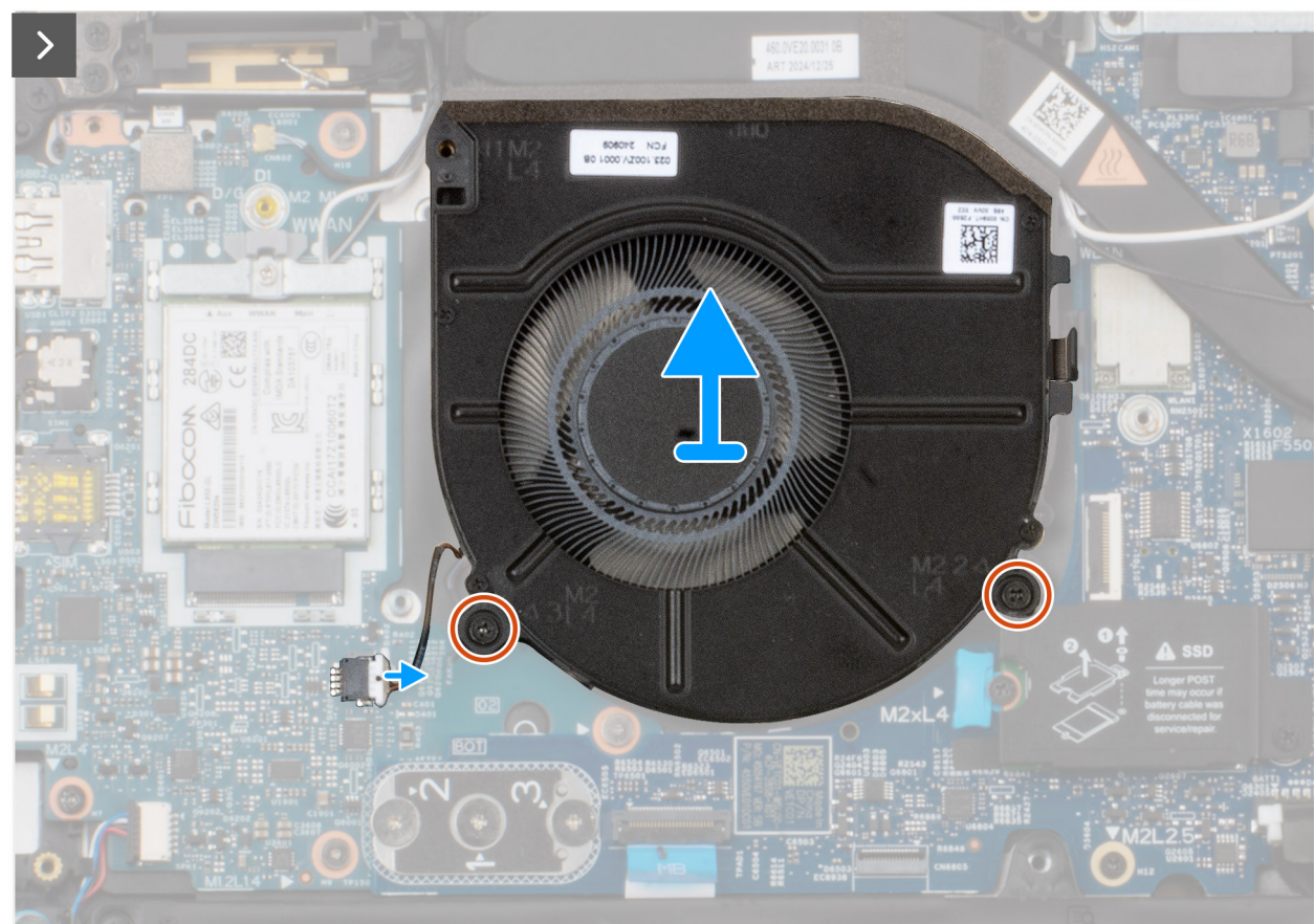
Figure 30. Removing the fan
