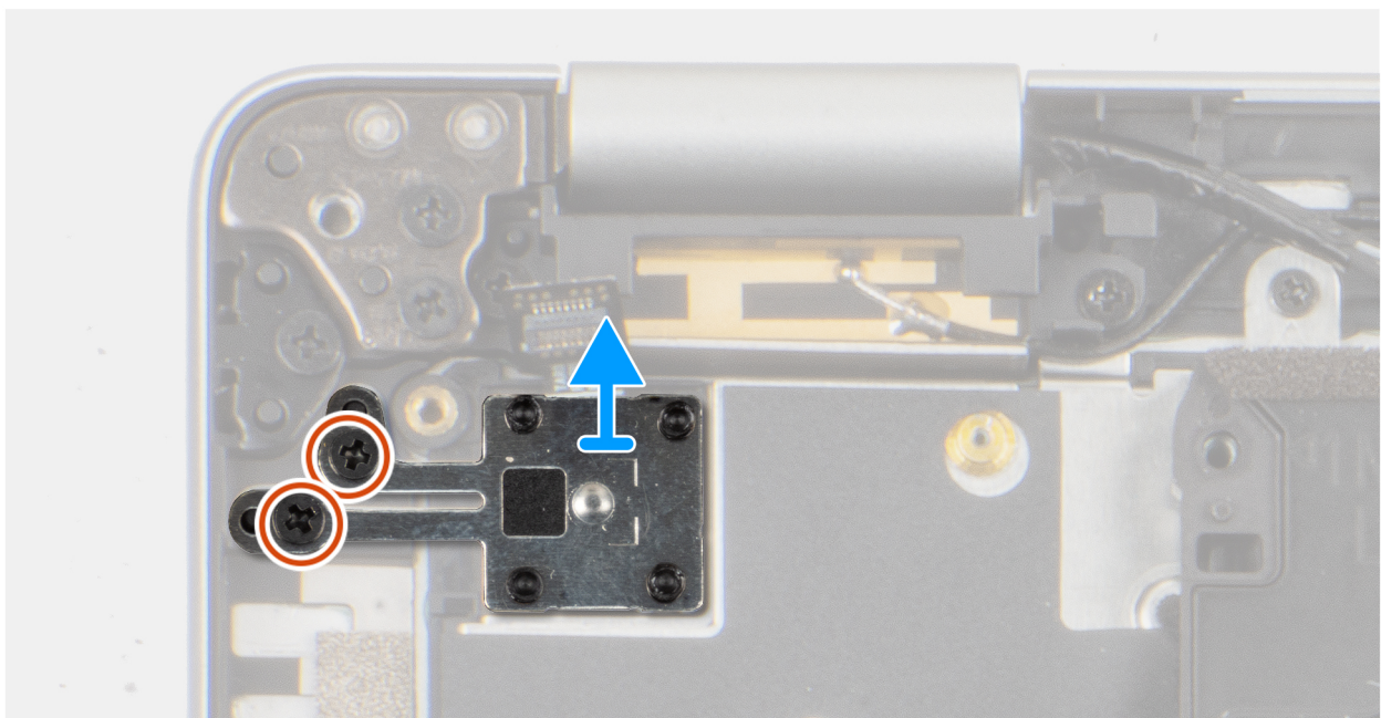
Figure 47. Removing the power button with optional fingerprint reader
