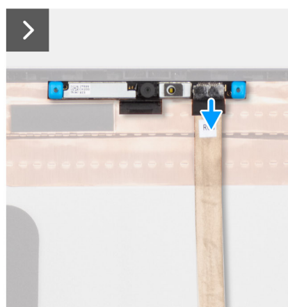
Figure 71. Installing the display cable
