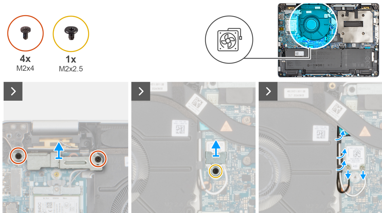
Figure 29. Removing the fan
