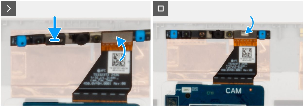
Figure 39. Installing the camera module display cable
