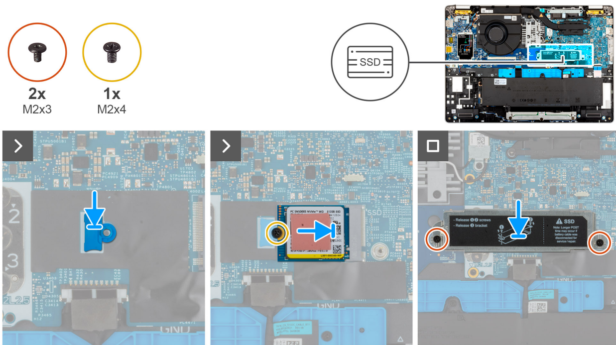
Figure 13. Installing the M.2 2230 SSD
