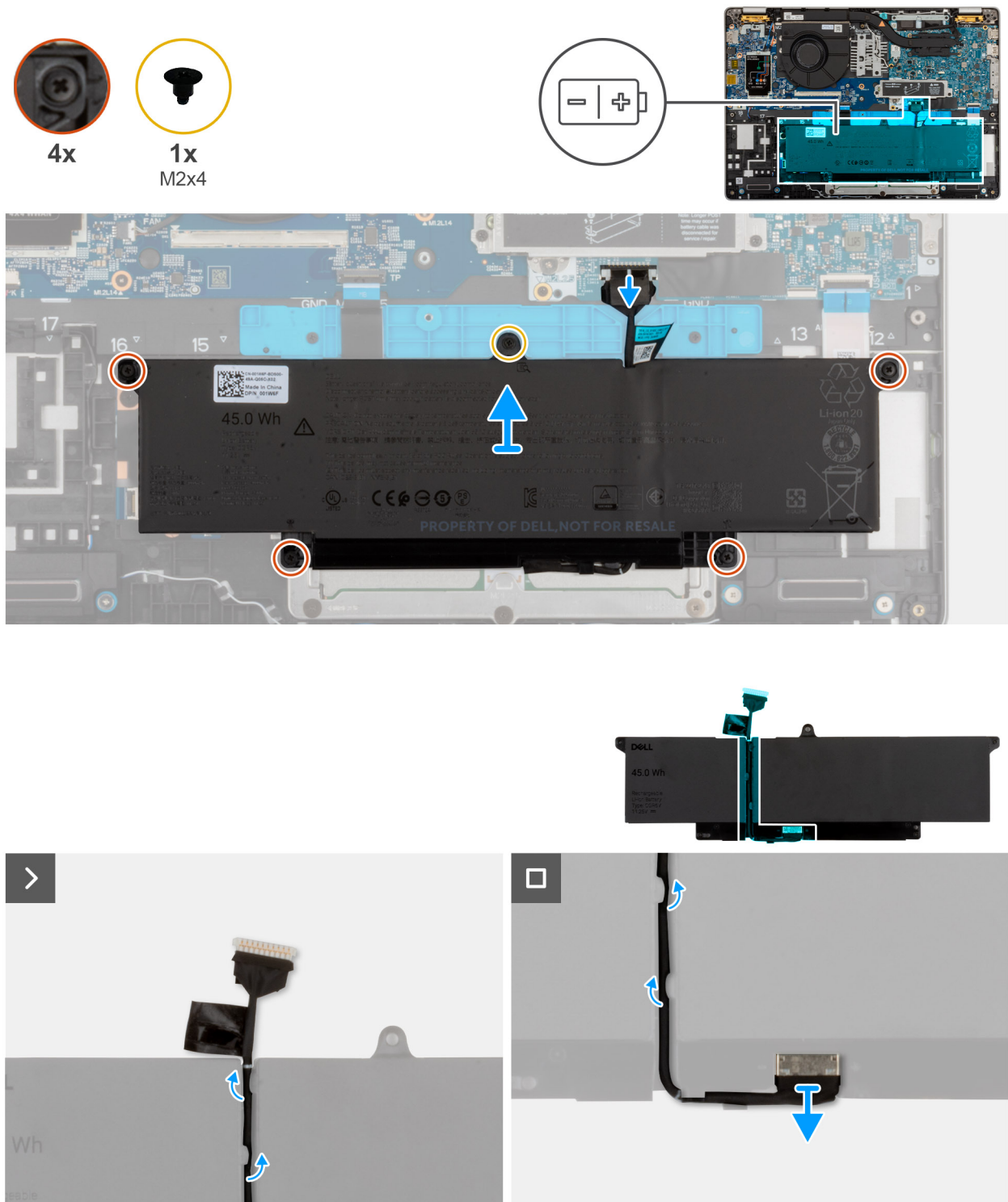
Figure 8. Removing the battery
