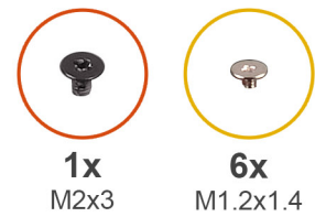
Figure 56. Removing the I/O board
