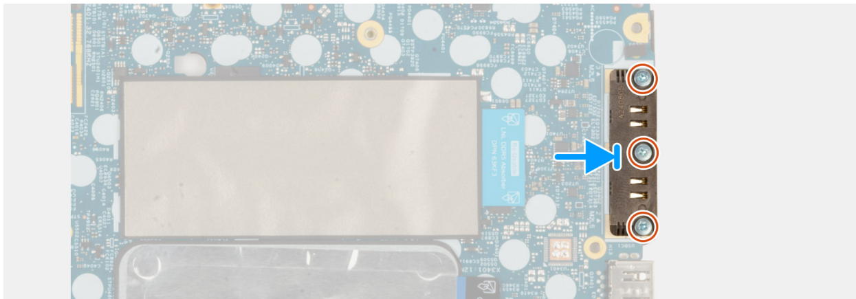
Figure 53. Installing the USB-C Connector Module
