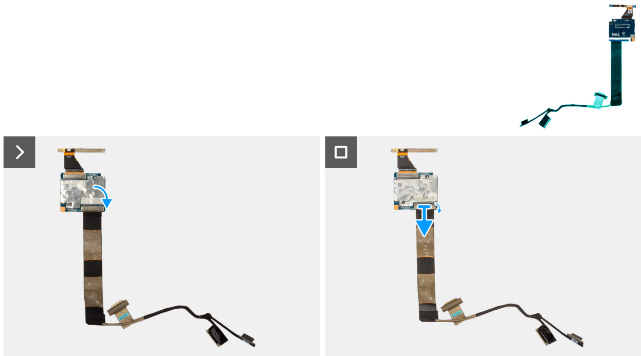
Figure 36. Removing the display cable
