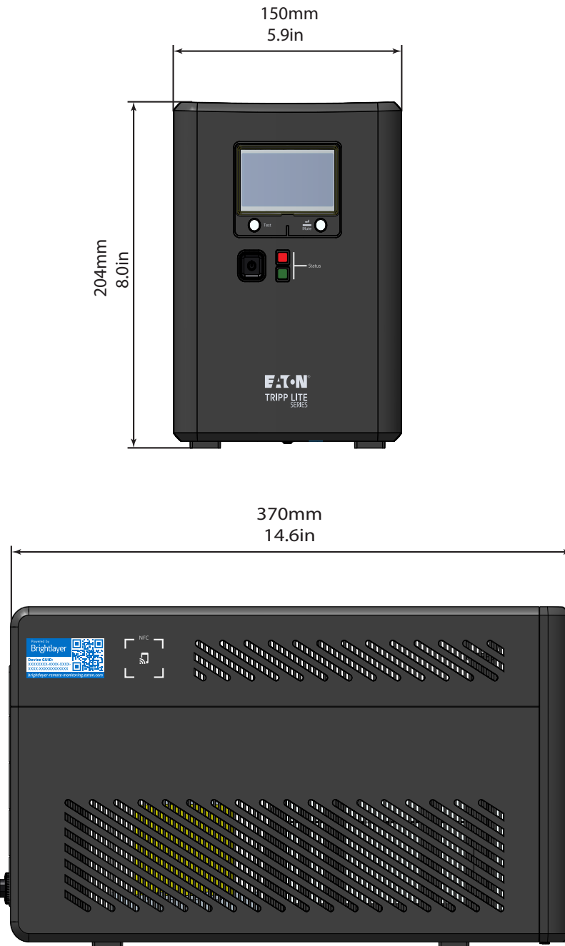
Figure 1. SMART750LCDTNC/SMART1000LCDTNC/SMART1500LCDTXC Dimensiones
