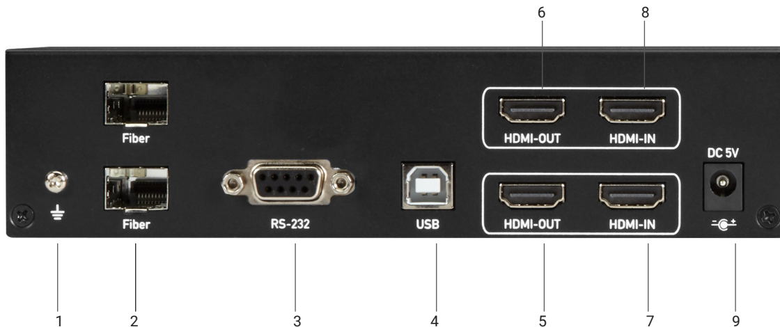
FIGURE 2-7. HDMI DUAL-HEAD FIBER TRANSMITTER BACK PANEL
