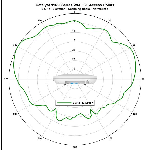
Figure 14: CW9162I - Scanning Radio-Normalized Radiation Pattern (6-GHz Elevation)
