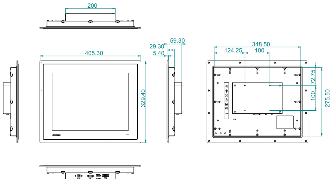
Figure 1.2 FPM-815S Dimensions
