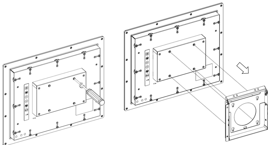
Figure 2.2 Wall Mounting
