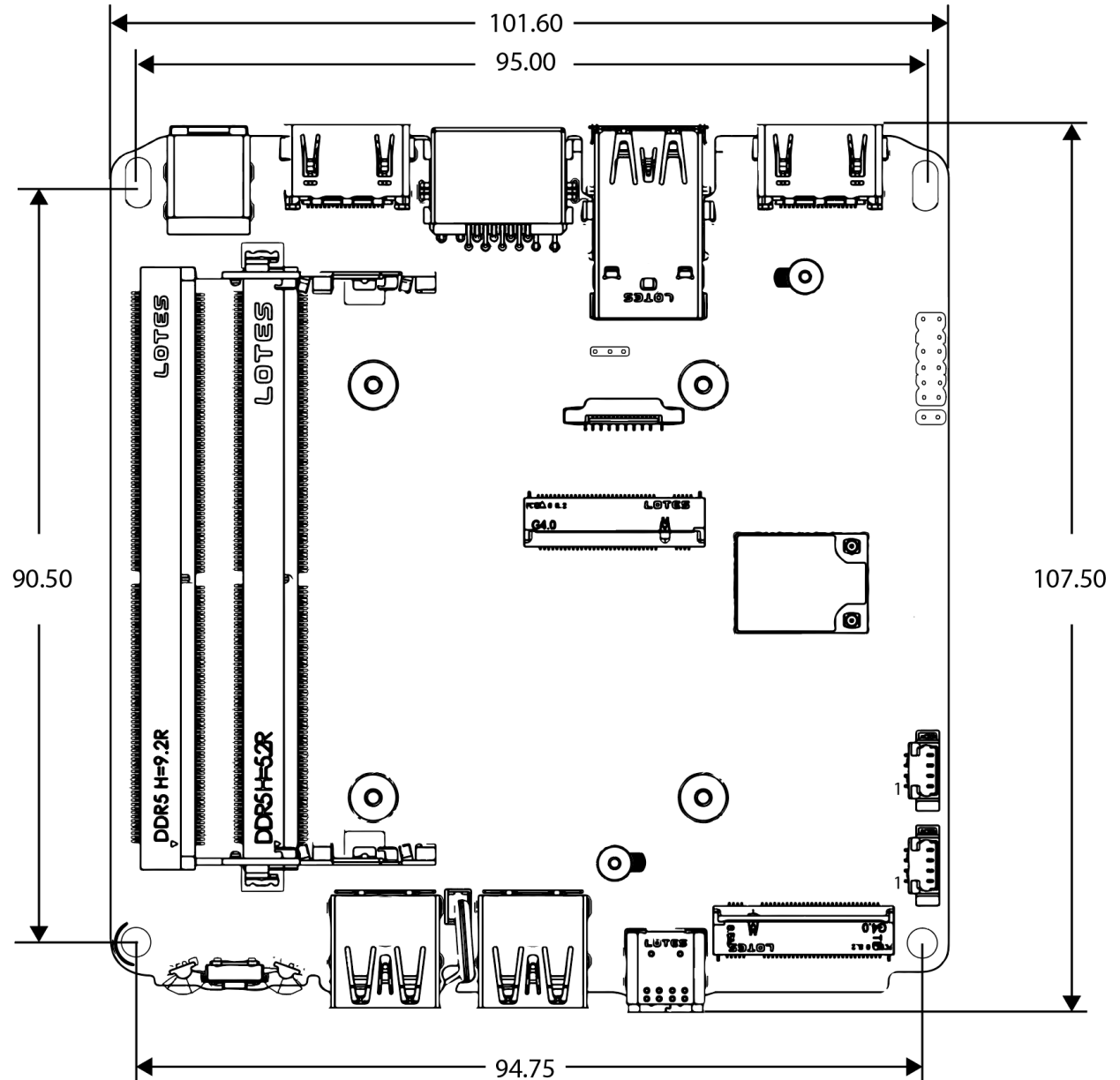
Figure 17. Board Dimensions
