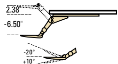
KSFK-21 - $266 Slim Fit Keyboard Support Mechanism 7.5w x 17.5d x 4.75h
