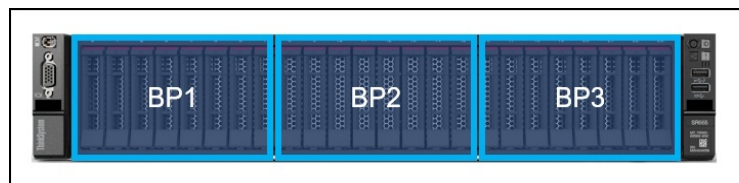
Figure 11. Backplane numbering
