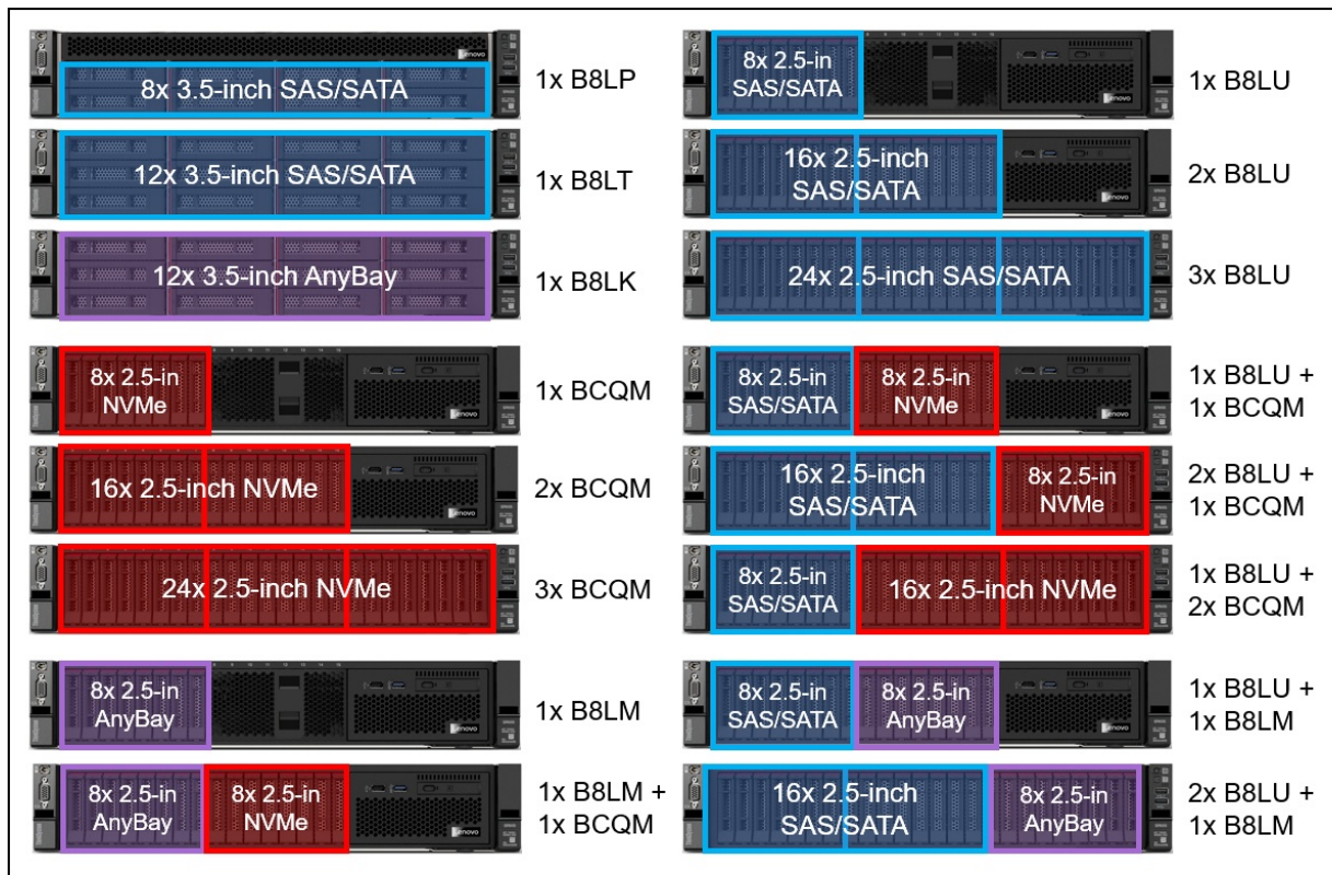
Figure 7. SR665 front drive bay configurations
