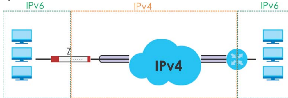
Figure 280 IPv6-in-IPv4 Tunnel
