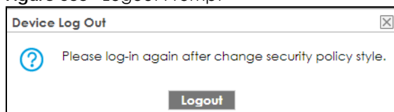
Figure 533 Logout Prompt
