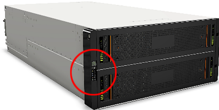
Figure 2-14 Control panel
