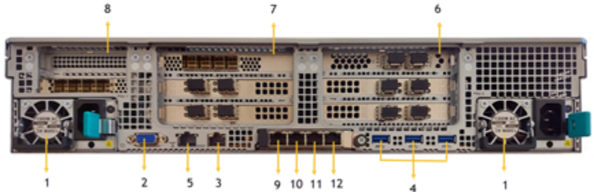
Figure 1-4 Appliance rear panel and connectors
