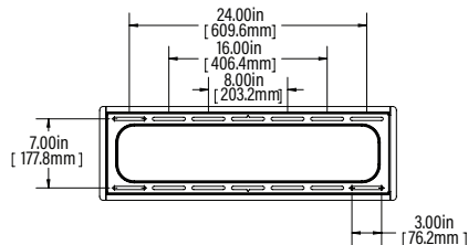
WALL PLATE
