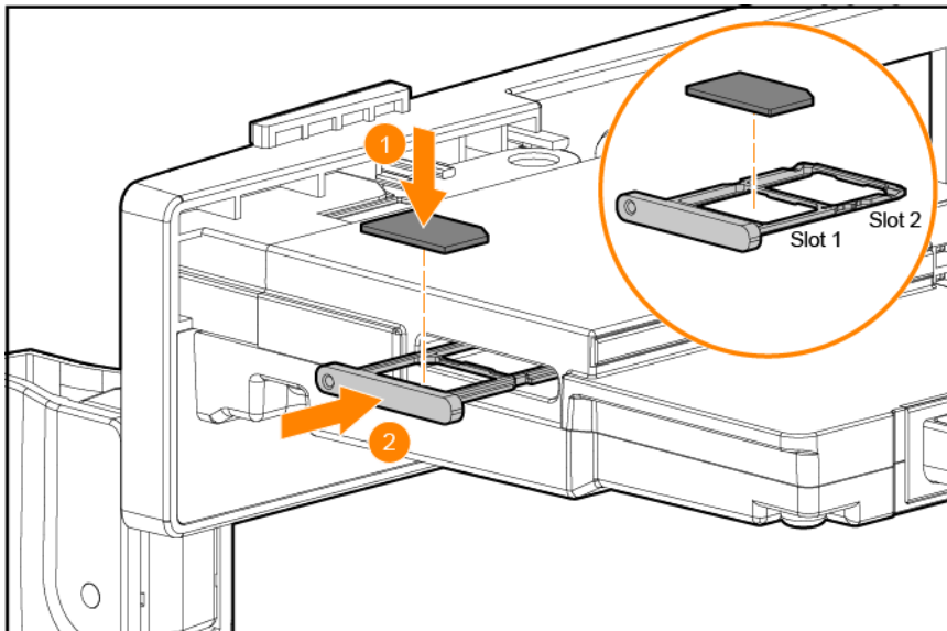
Figure 10 Inserting a SIM Card
