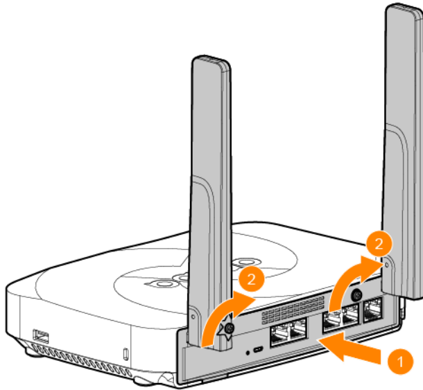
Figure 11 Installing Cellular Module onto Access Point
