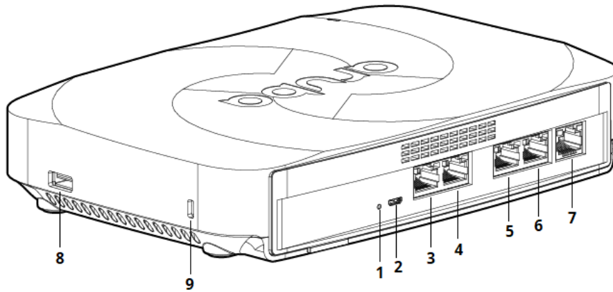
Figure 3 600R Series Rear and Side View
