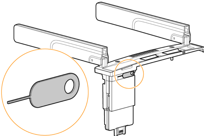
Figure 8 SIM Ejector Needle Location
