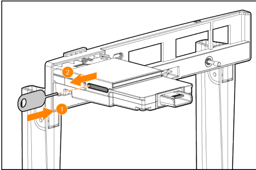
Figure 9 Opening the SIM Card Tray
