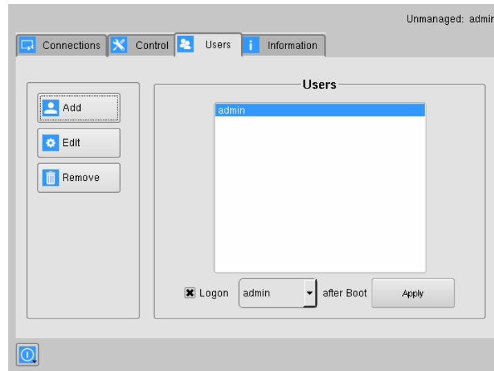
FIGURE 8-30. USER SCREENS
