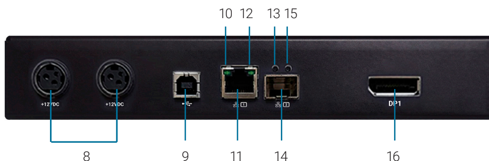
FIGURE 5-14. REAR VIEW OF THE EMERALD PE TRANSMITTER, SINGLE-HEAD (EMD2000PE-DP-R)
