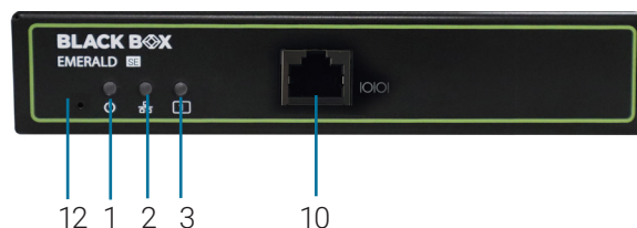
FIGURE 5-25. FRONT VIEW OF THE EMERALD SE R2 DVI TRANSMITTER, DUAL-HEAD (EMD2000SE-T-R2)
