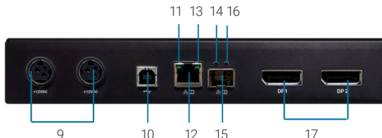
FIGURE 5-16. BACK VIEW OF THE EMERALD PE TRANSMITTER, DUAL-HEAD (EMD2002PE-DP-R)
