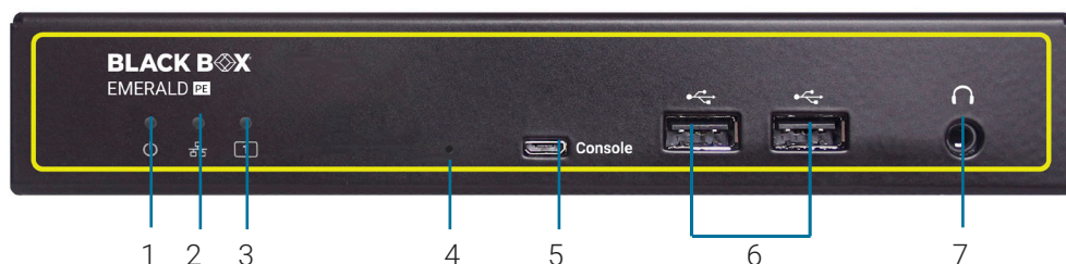
FIGURE 5-13. FRONT VIEW OF THE EMERALD PE TRANSMITTER, SINGLE-HEAD (EMD2000PE-DP-R)
