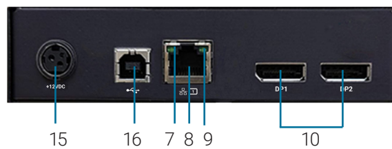
FIGURE 5-8. REAR VIEW OF EMERALD SE DP RECEIVER, DUAL-HEAD (EMD2002SE-DP-R)
