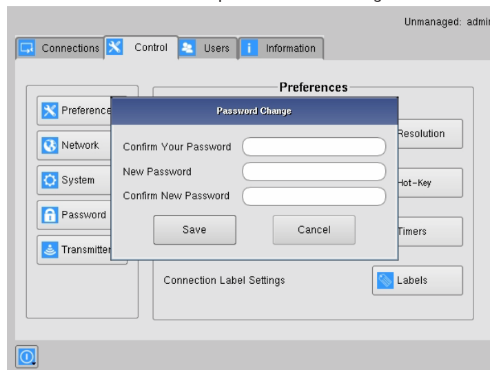
FIGURE 8-25. PASSWORD CHANGE
