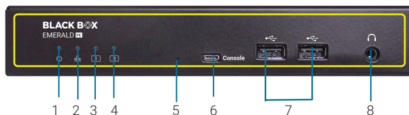
FIGURE 5-15. FRONT VIEW OF THE EMERALD PE TRANSMITTER, DUAL-HEAD (EMD2002PE-DP-R)
