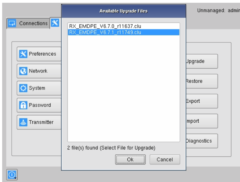
FIGURE 8-22. UPGRADE FILES
