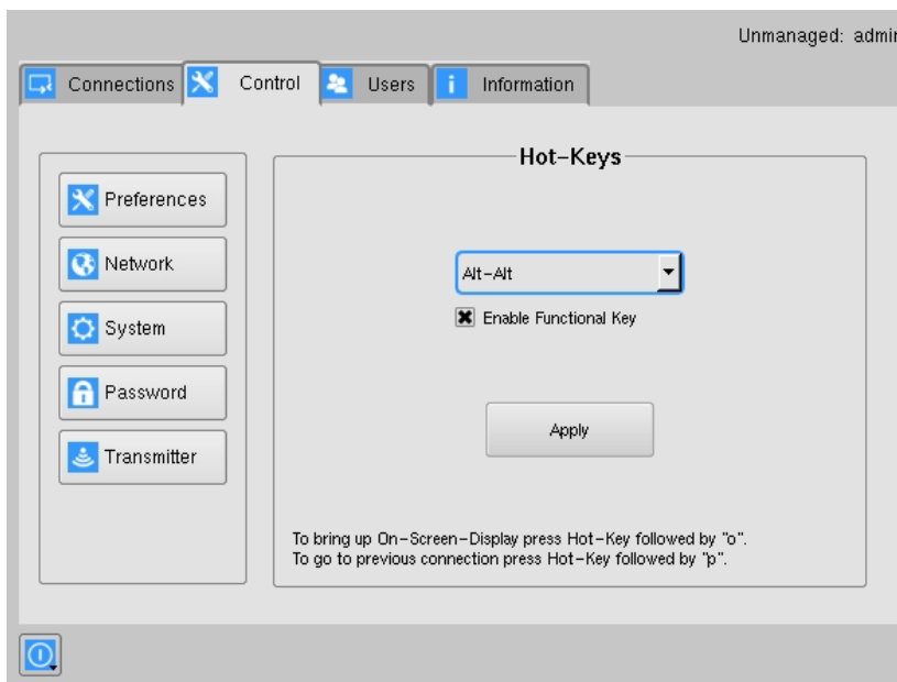
FIGURE 8-14. HOT-KEY DEFINITION
