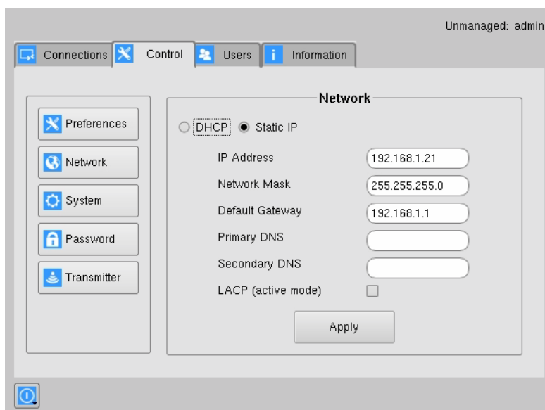
FIGURE 8-21. NETWORK SETTINGS
