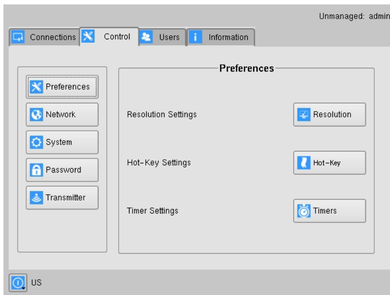
FIGURE 8-12. CONTROL TAB
