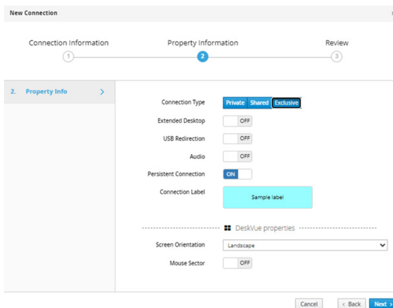
FIGURE 8-9. CONNECTION PARAMETERS
