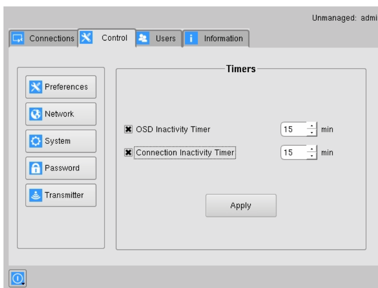
FIGURE 8-15. TIMER SETTINGS
