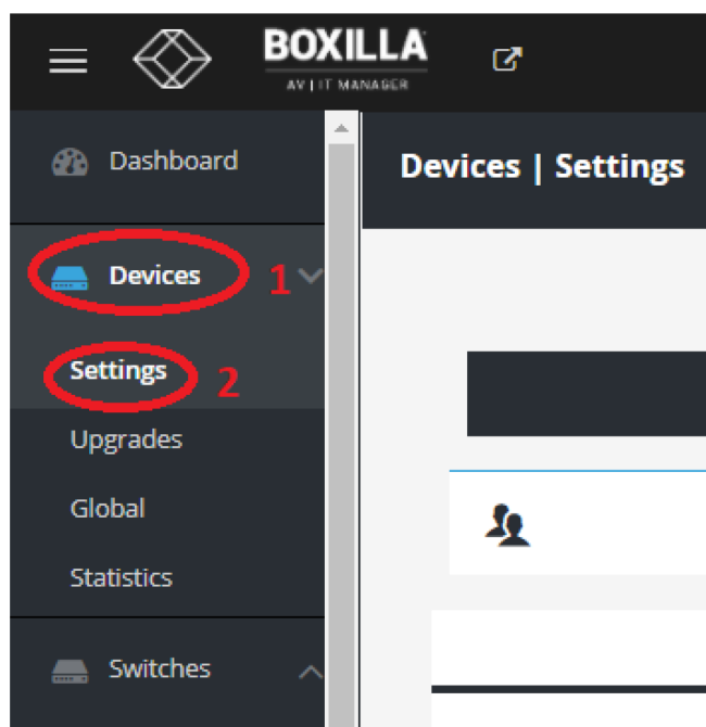
FIGURE C-1. SETTINGS SCREEN
