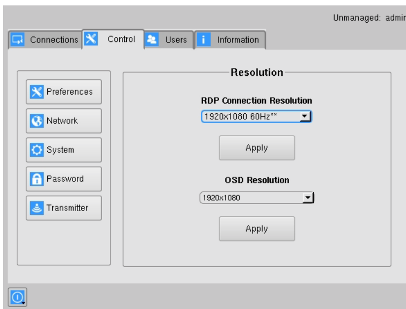
FIGURE 8-13. RESOLUTION SCREEN
