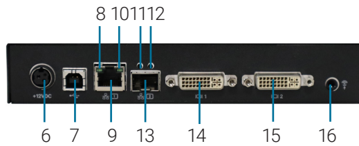
FIGURE 5-38. REAR VIEW OF EMD2002PE-T-R2
