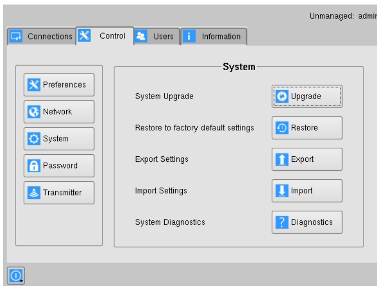
FIGURE 8-22. SYSTEM SCREEN
