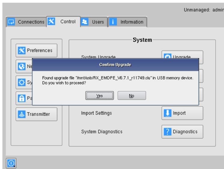
FIGURE 8-24. CONFIRMATION SCREEN
