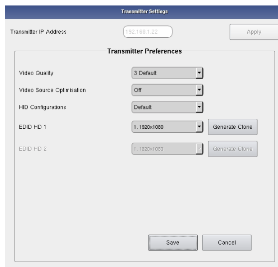
FIGURE 8-28. TRANSMITTER PREFERENCES
