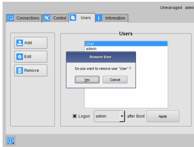
FIGURE 8-33. REMOVE USER
