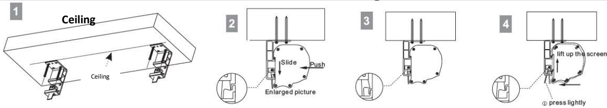
Screen-to-ceiling installation with brackets
