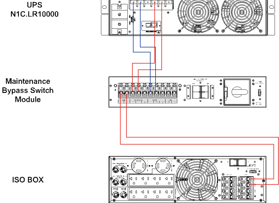
Wiring diagram to connect UPS, transformer box and maintenance bypass
