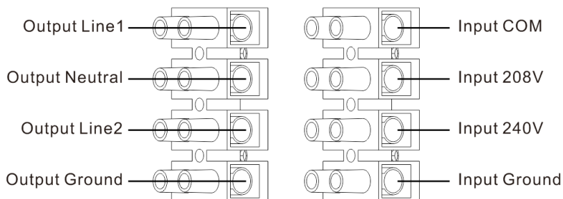
Terminal block wiring diagram of TRANSFORMER BOX
