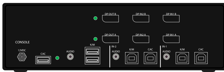
Figure 1-2: KVS4-2002VX Rear panel
