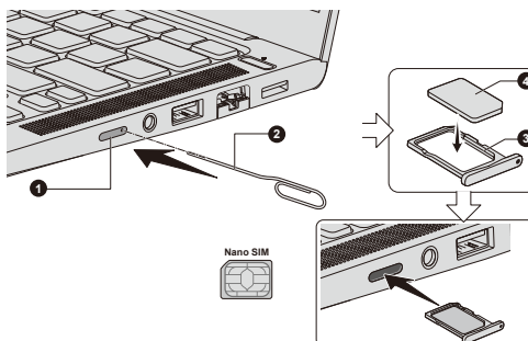
Figure 4-5 Installing the SIM card
