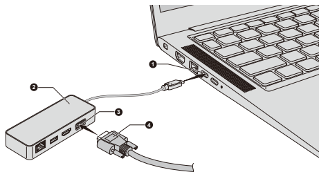
Figure 4-9 Connecting the RGB cable to the RGB monitor port
