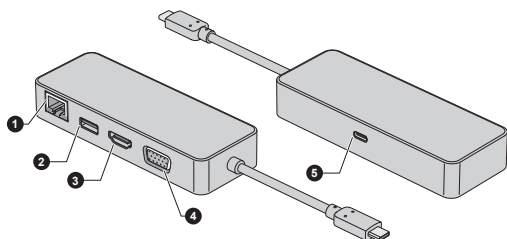
Figure 4-7 USB-C™ to HDMI™/VGA Travel Adapter
