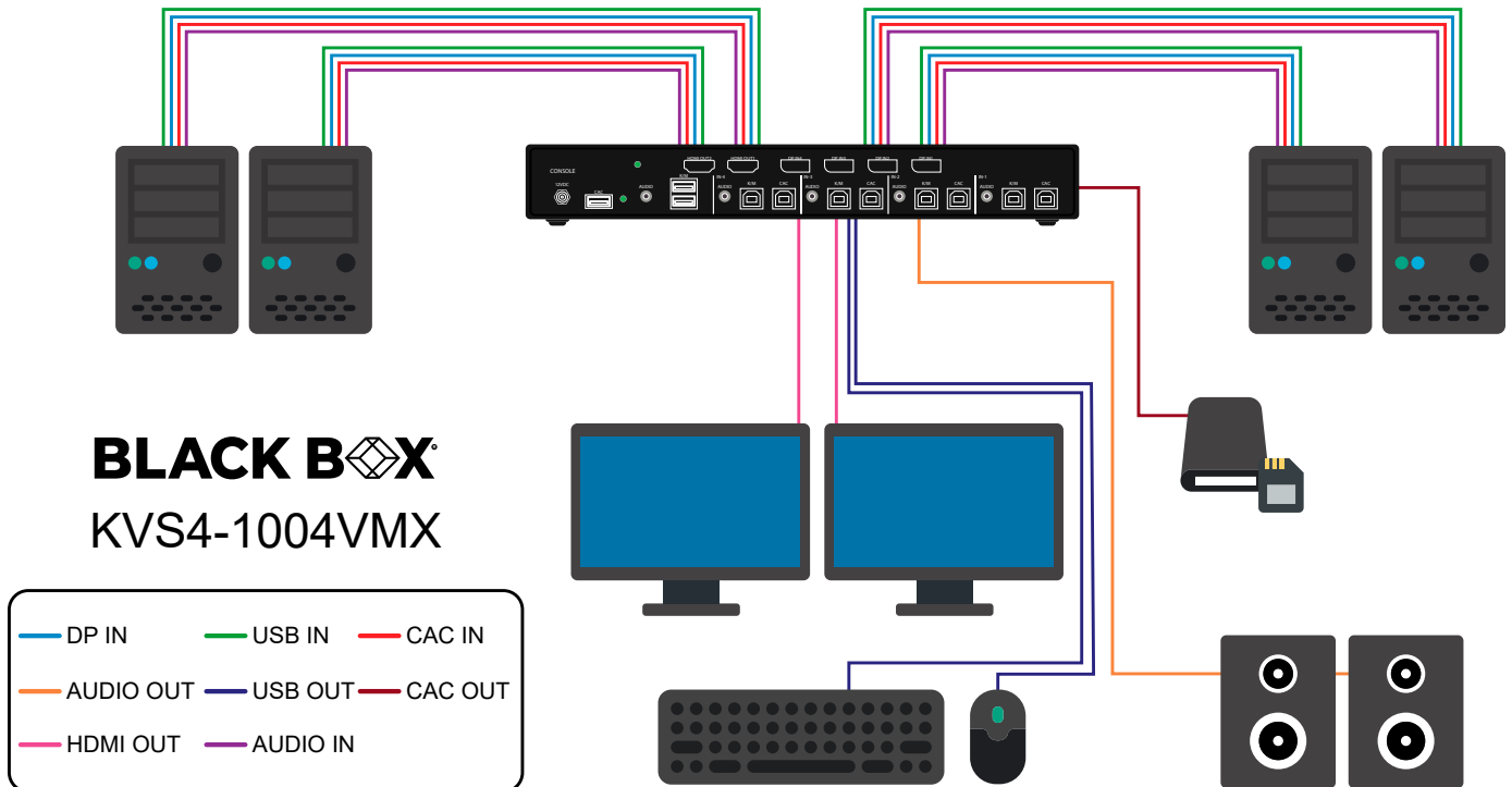
Figure 1-3: KVS4-1004VMX
