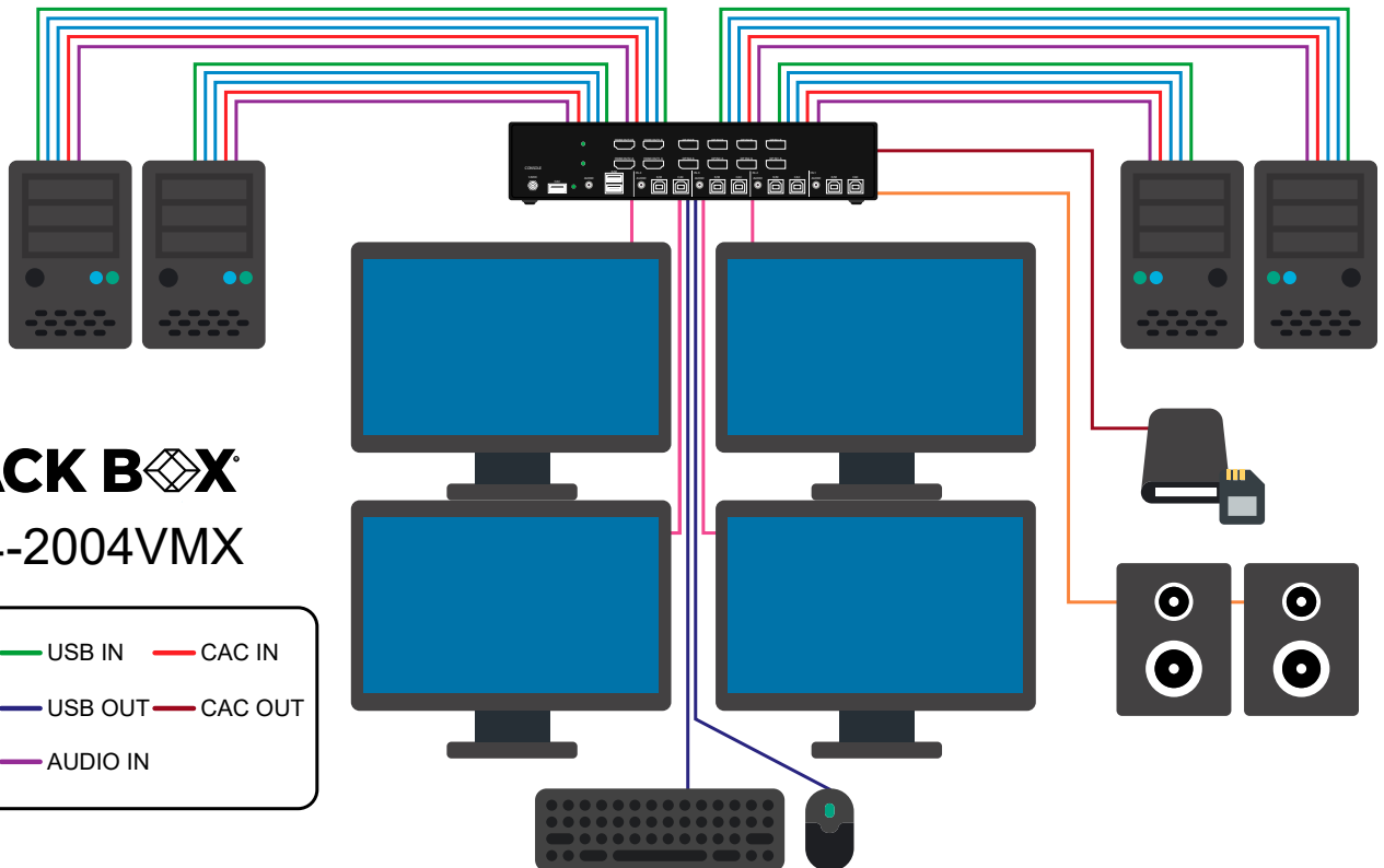
Figure 1-7: KVS4-2004VMX
