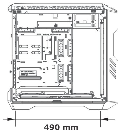
Maximum length for Graphics card
