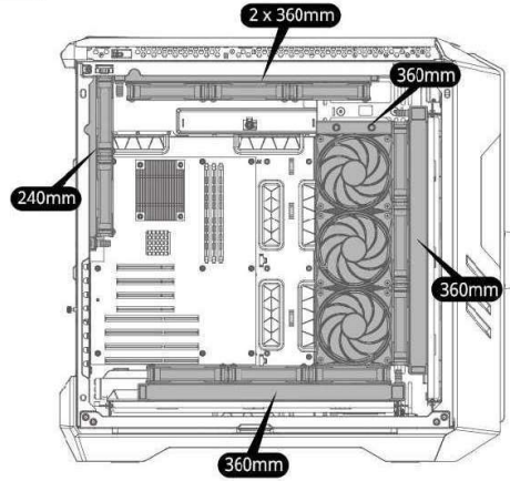
D Maximum liquid cooling build
