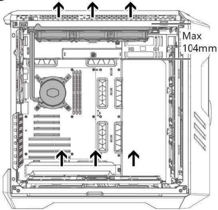
C Recommended single radiator position
