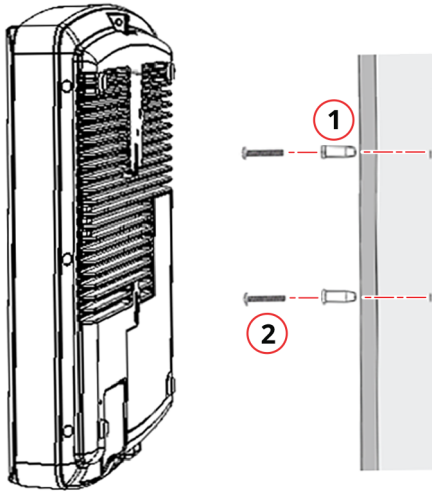
FIGURE 9 Flat Surface Mounting
