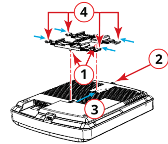
FIGURE 7 Attaching the T-bar Bracket to the AP
