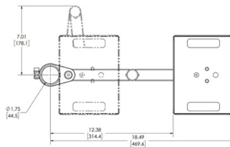
Printer Mount - 16" Folding Extension Arm - Medium Tray
