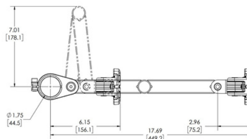
Payment Terminal Mount on 16" Folding Extension Arm
