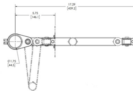
Monitor Mount on 16" Folding Extension Arm
