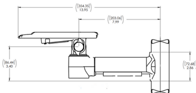
Payment Terminal Mount with MM-10-204
