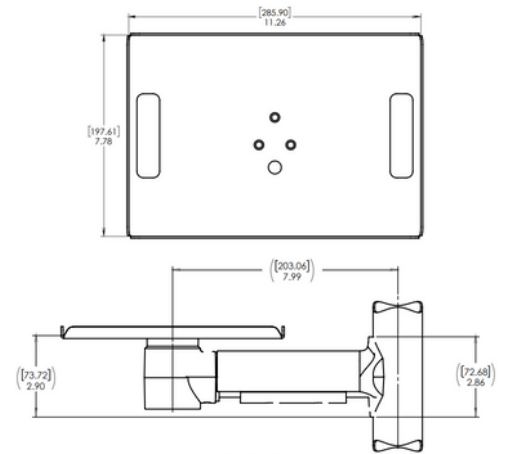
Large Printer Mount
