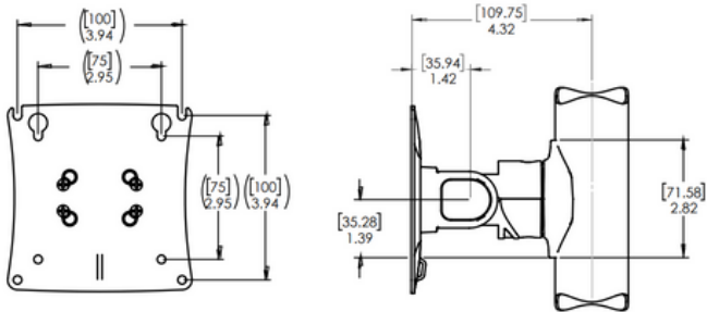
Single Pivot Monitor Mount
