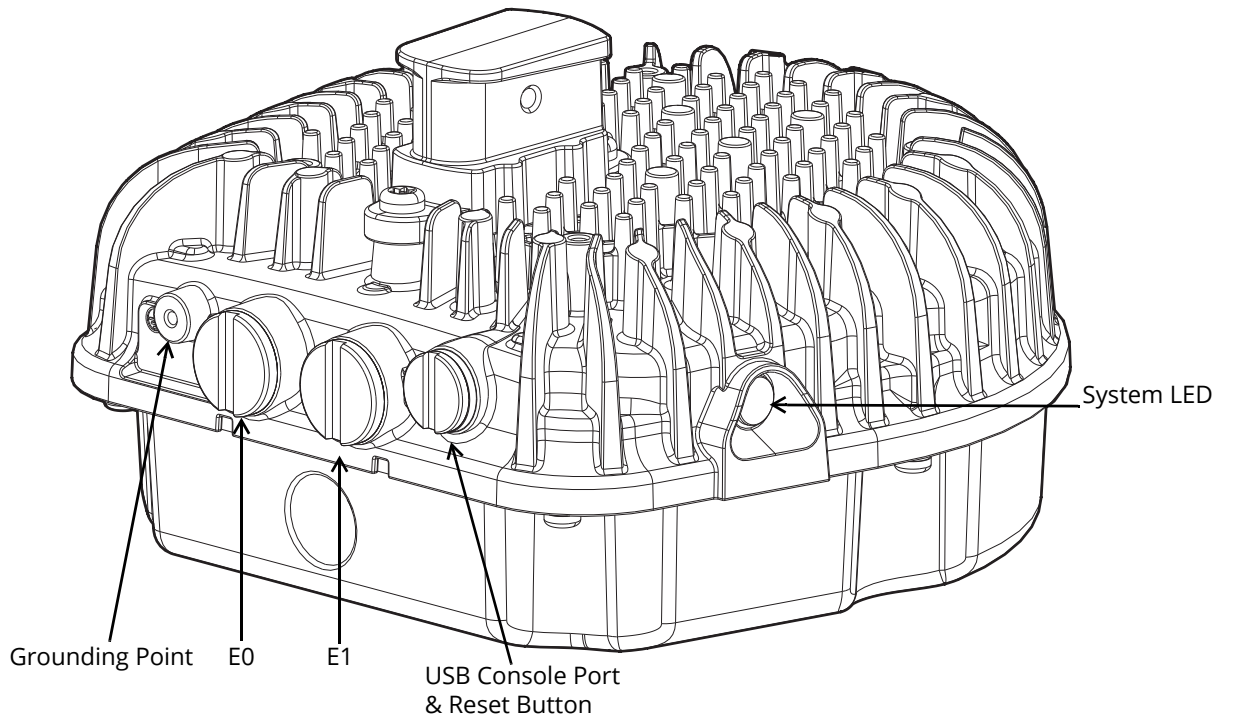
Figure 4 AP-577EX Rear View
