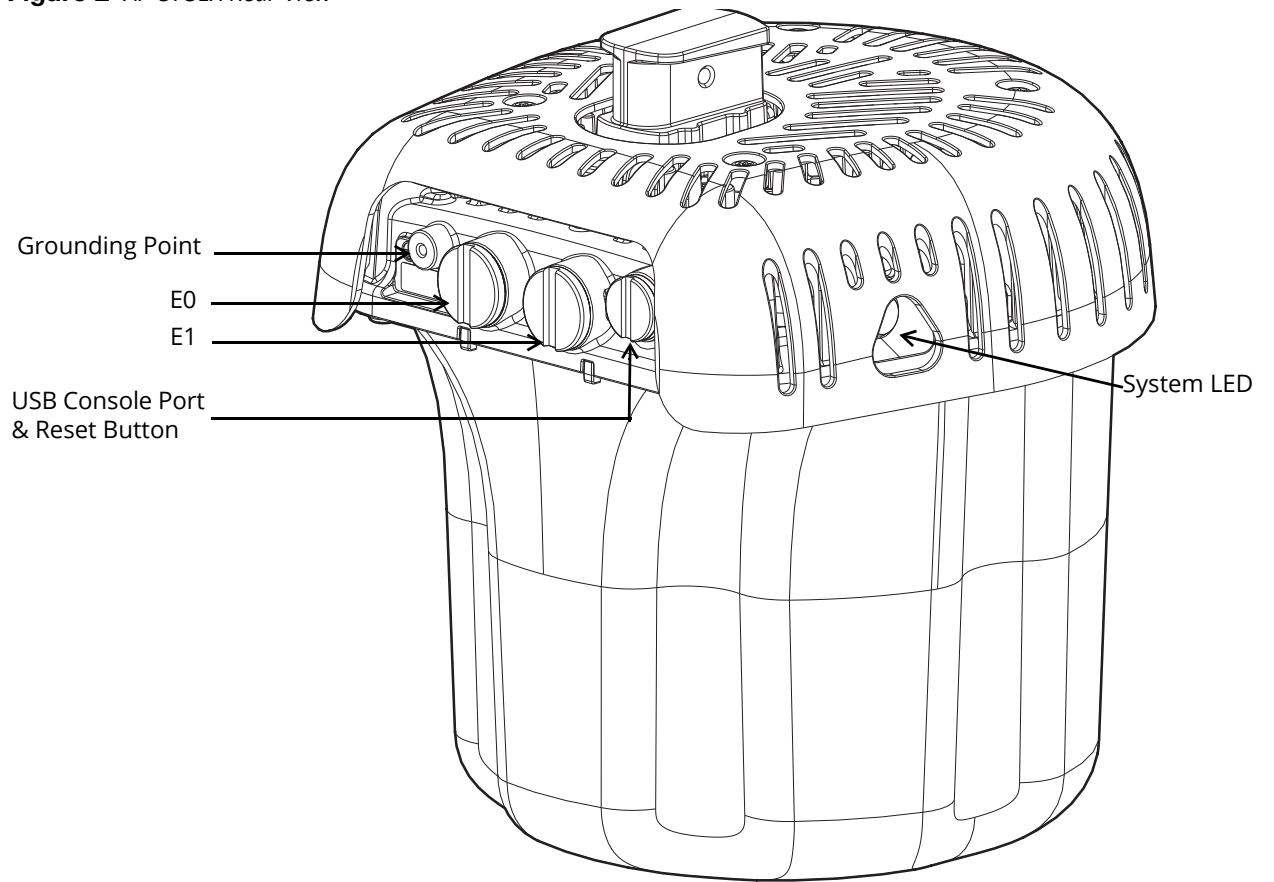
Figure 2 AP-575EX Rear View
