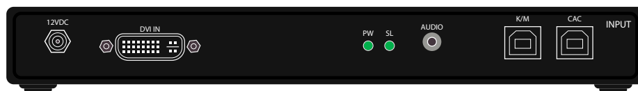
Figure 1-2: KVS4-8001DX Rear panel
