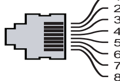
RJ-45 Female Pin-Out
