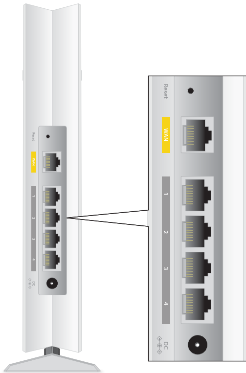
Figure 5. Back panel, model WAX206
