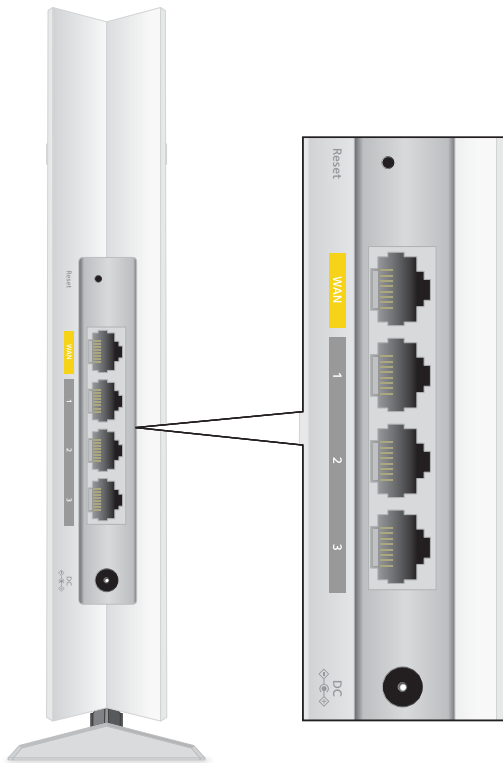
Figure 2. Back panel, model WAX202
