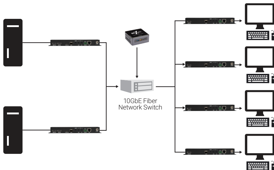
FIBER KVM SWITCH CONFIGURATION
