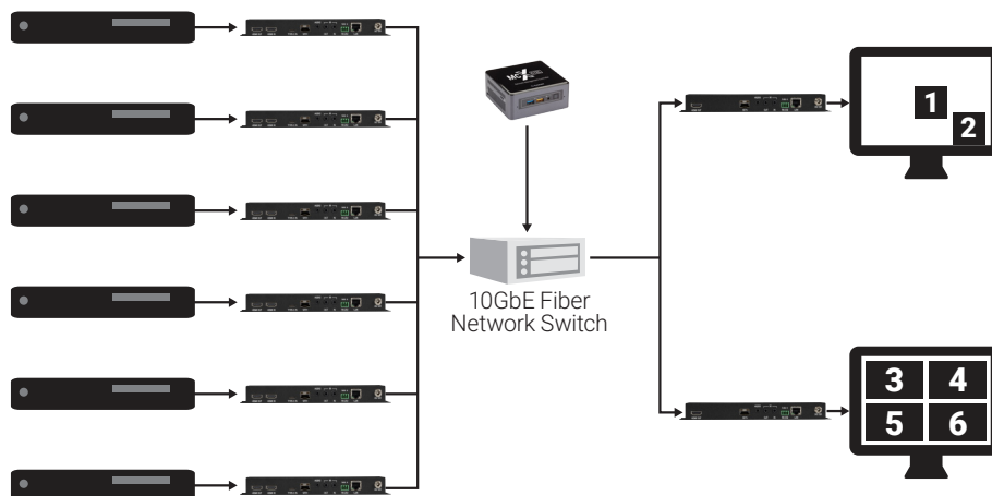
FIBER MULTIVIEW (PIP/POP/QUAD/ETC.) CONFIGURATION
