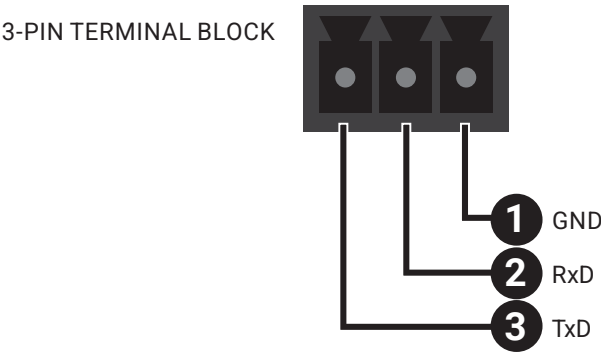
3-PIN TERMINAL BLOCK
