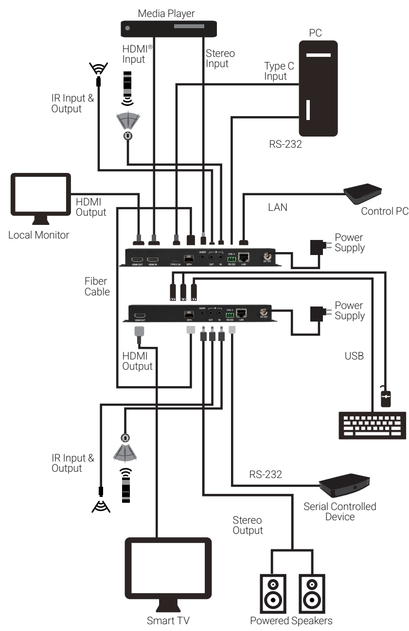
FIBER CONNECTION DIAGRAM
