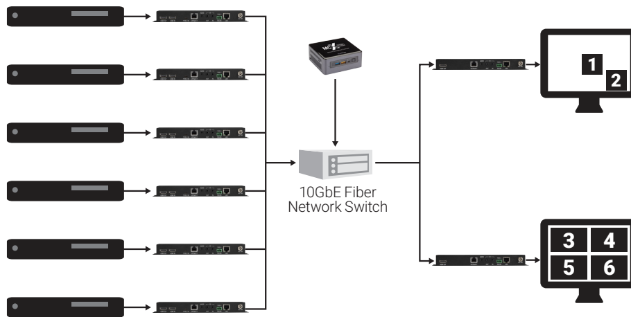
COPPER MULTIVIEW (PIP/POP/QUAD/ETC.) CONFIGURATION
