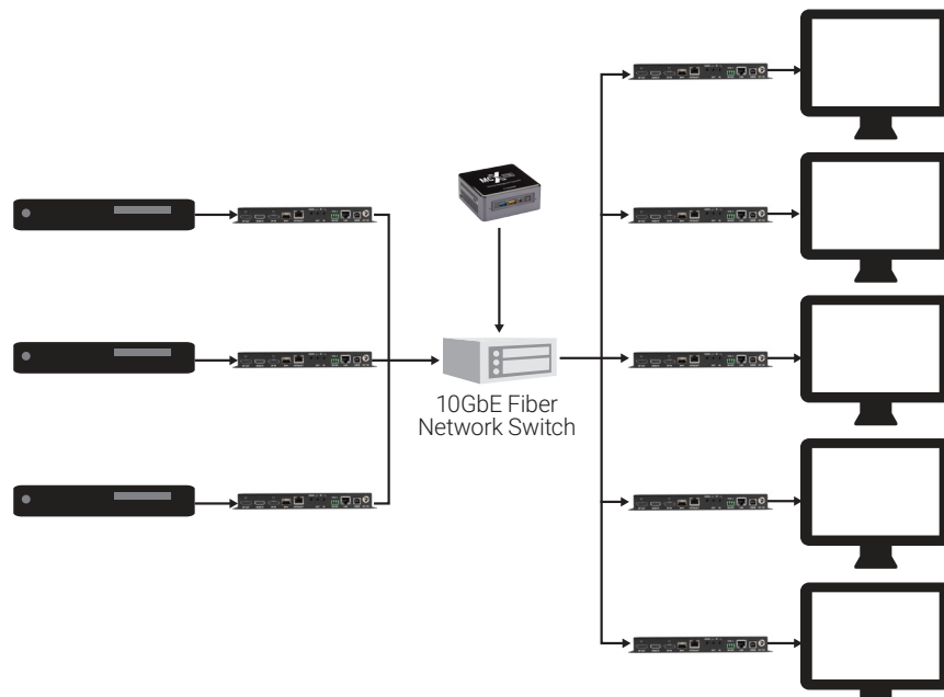
FIBER MATRIX CONFIGURATION
