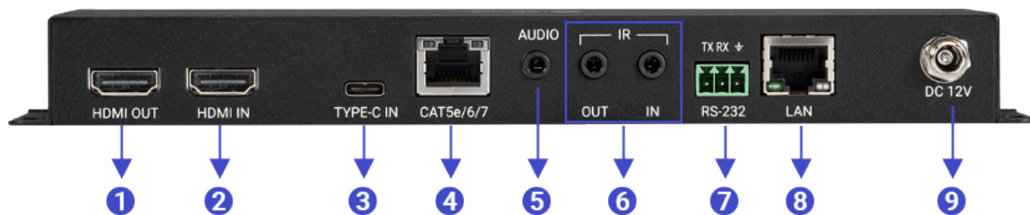
REAR PANEL (COPPER)
