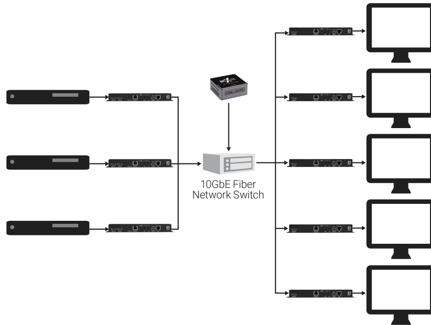
COPPER MATRIX CONFIGURATION
