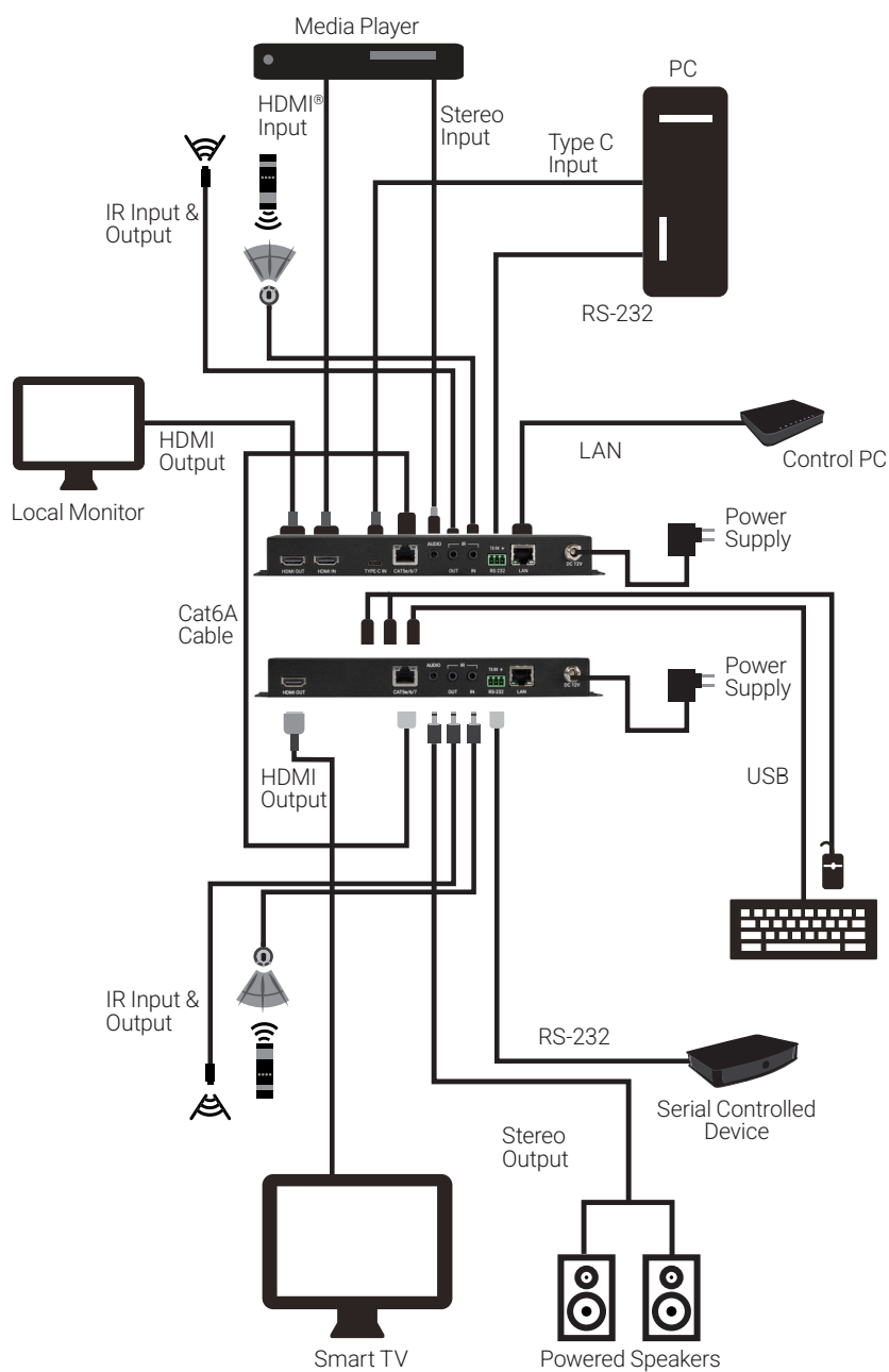
COPPER CONNECTION DIAGRAM
