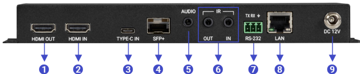
REAR PANEL (FIBER)
