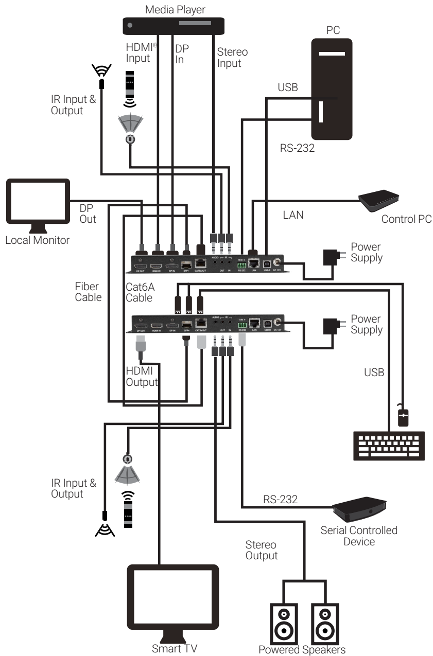
COPPER/FIBER CONNECTION DIAGRAM
