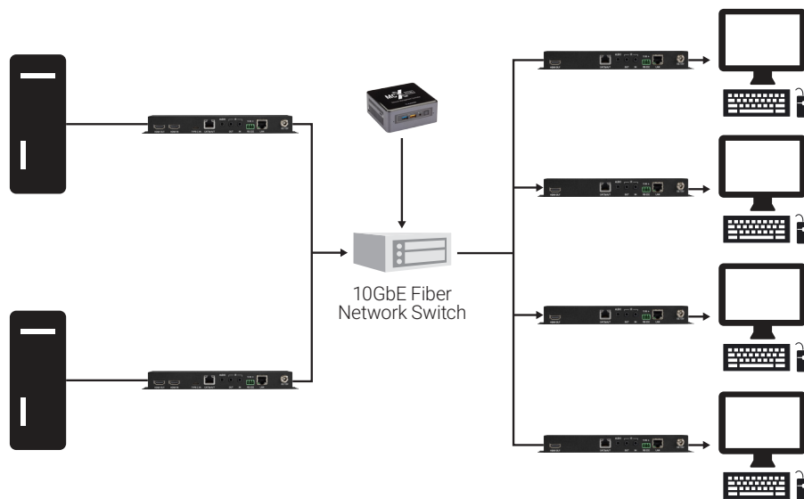
COPPER KVM SWITCH CONFIGURATION
