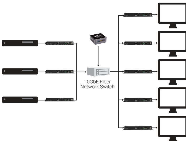
COPPER MATRIX CONFIGURATION
