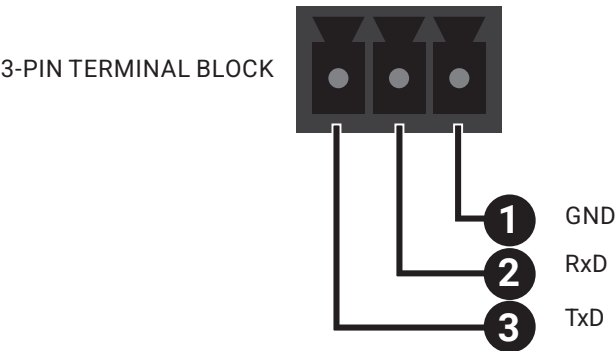
3-PIN TERMINAL BLOCK
