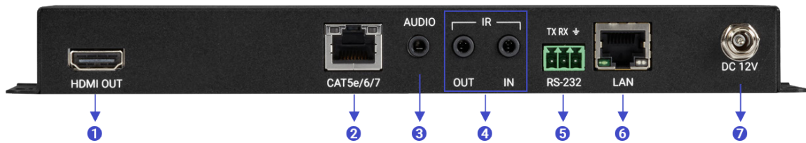
REAR PANEL (COPPER)
