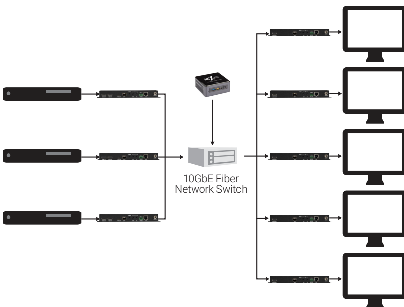
FIBER MATRIX CONFIGURATION
