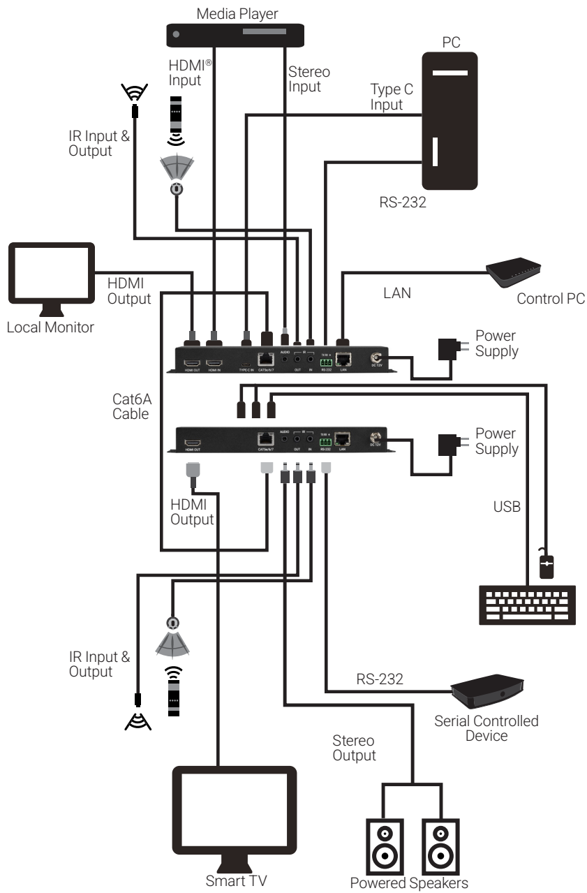
COPPER CONNECTION DIAGRAM
