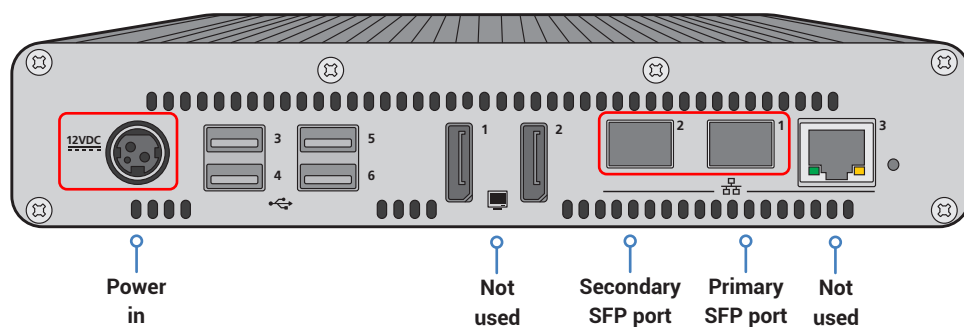
iPATH Agility Controller rear panel - In normal use only the SFP network and power connectors are used (ringed in red)
