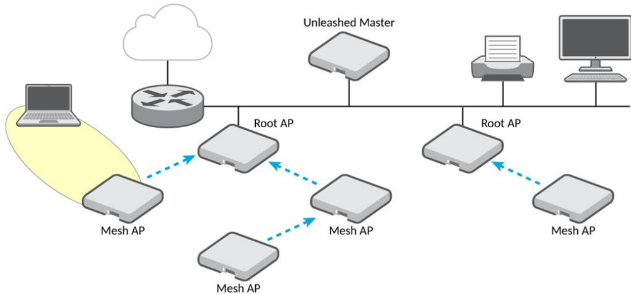
Figure 1. Mesh - standard topology
