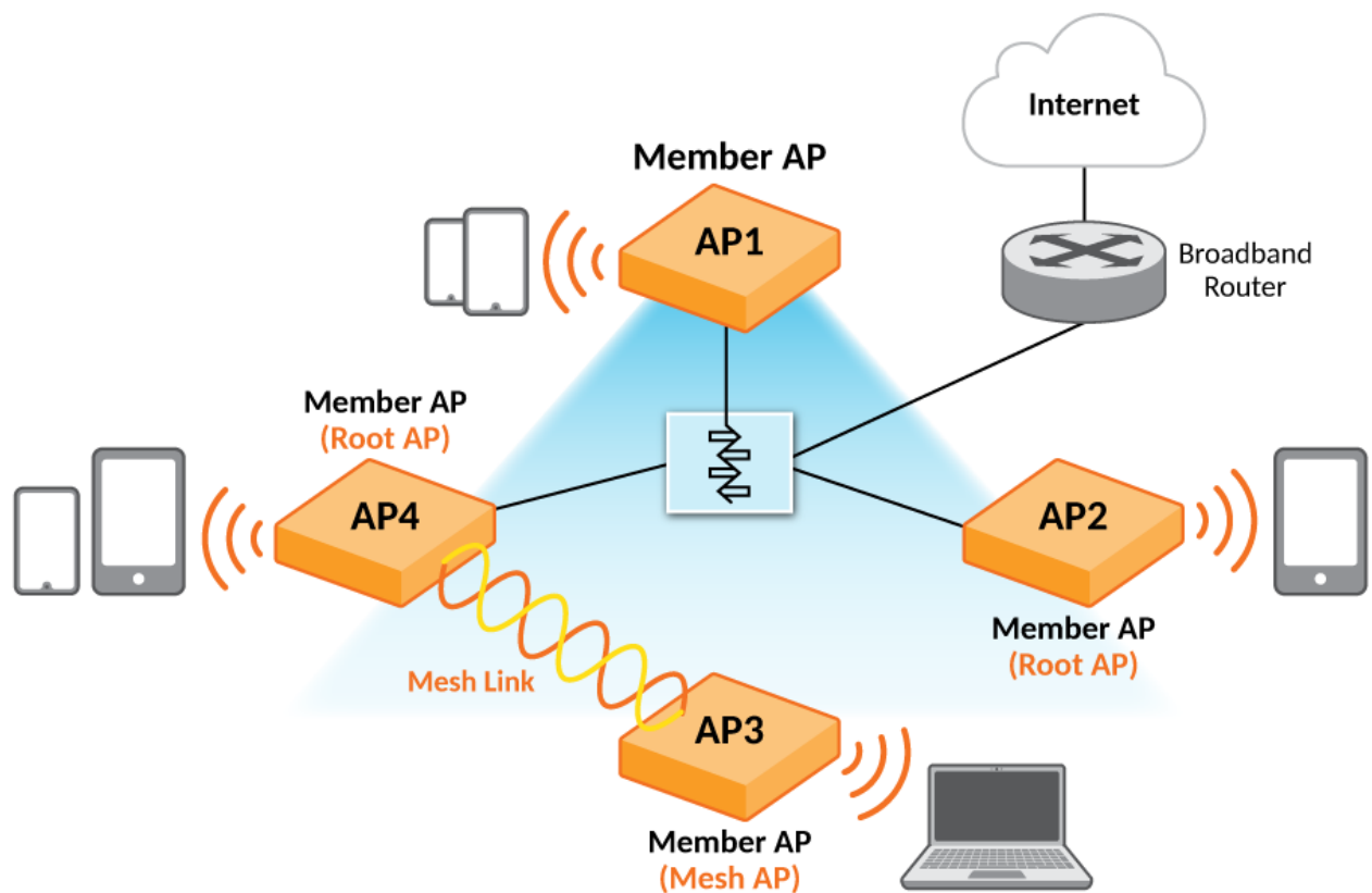
Figure 1. Basic Unleashed Network Topology
