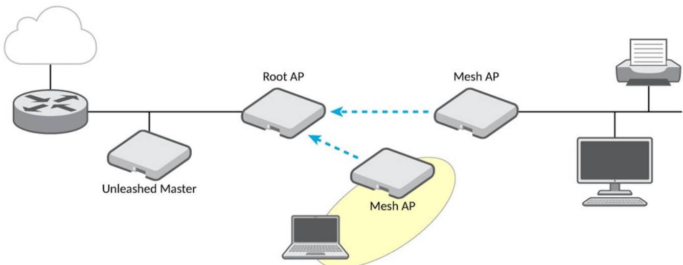
Figure 2. Mesh - wireless bridge topology
