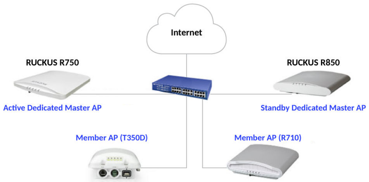
Figure 2. Basic Unleashed Dedicated Master Network Topology
