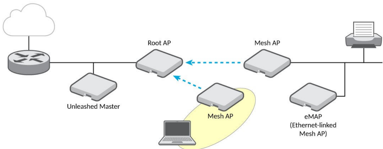
Figure 3. eMAP - Hybrid Mesh topology
