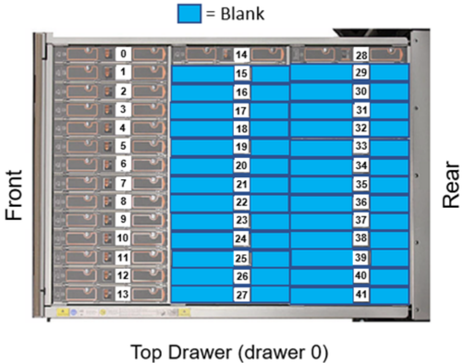
Figure 1-3 Half-populated storage shelf
