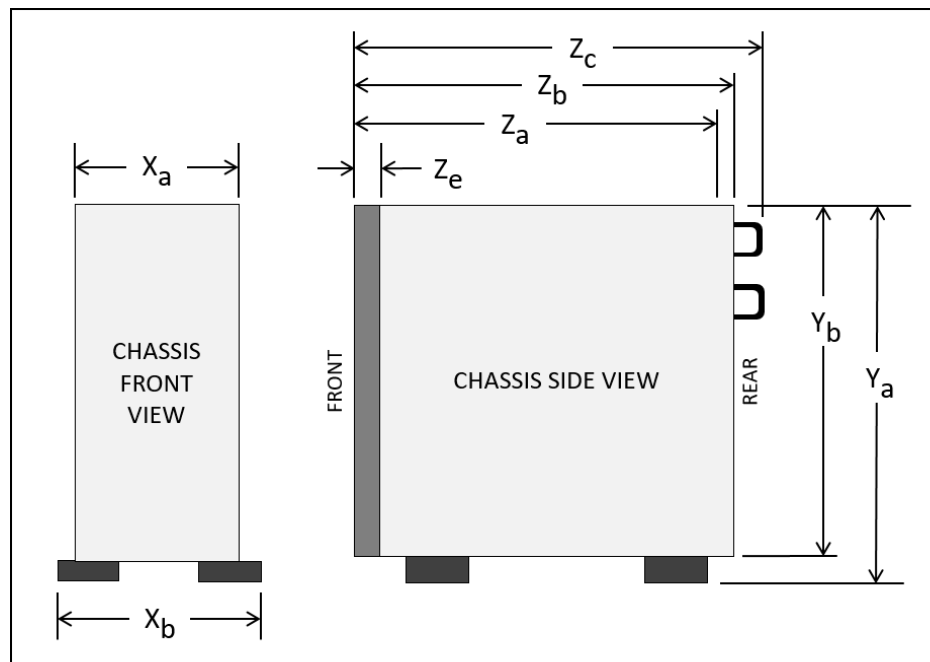
Figure 14. Server dimension
