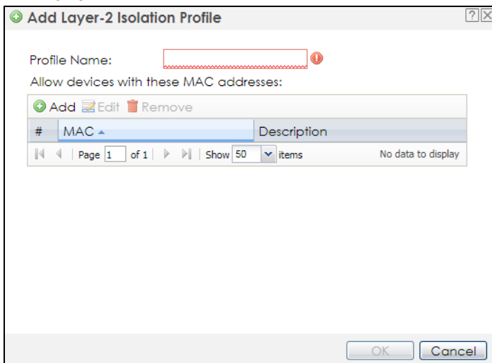
Figure 95 Configuration > Object > AP Profile > SSID > Layer-2 Isolation List > Add/Edit Layer-2 Isolation Profile
