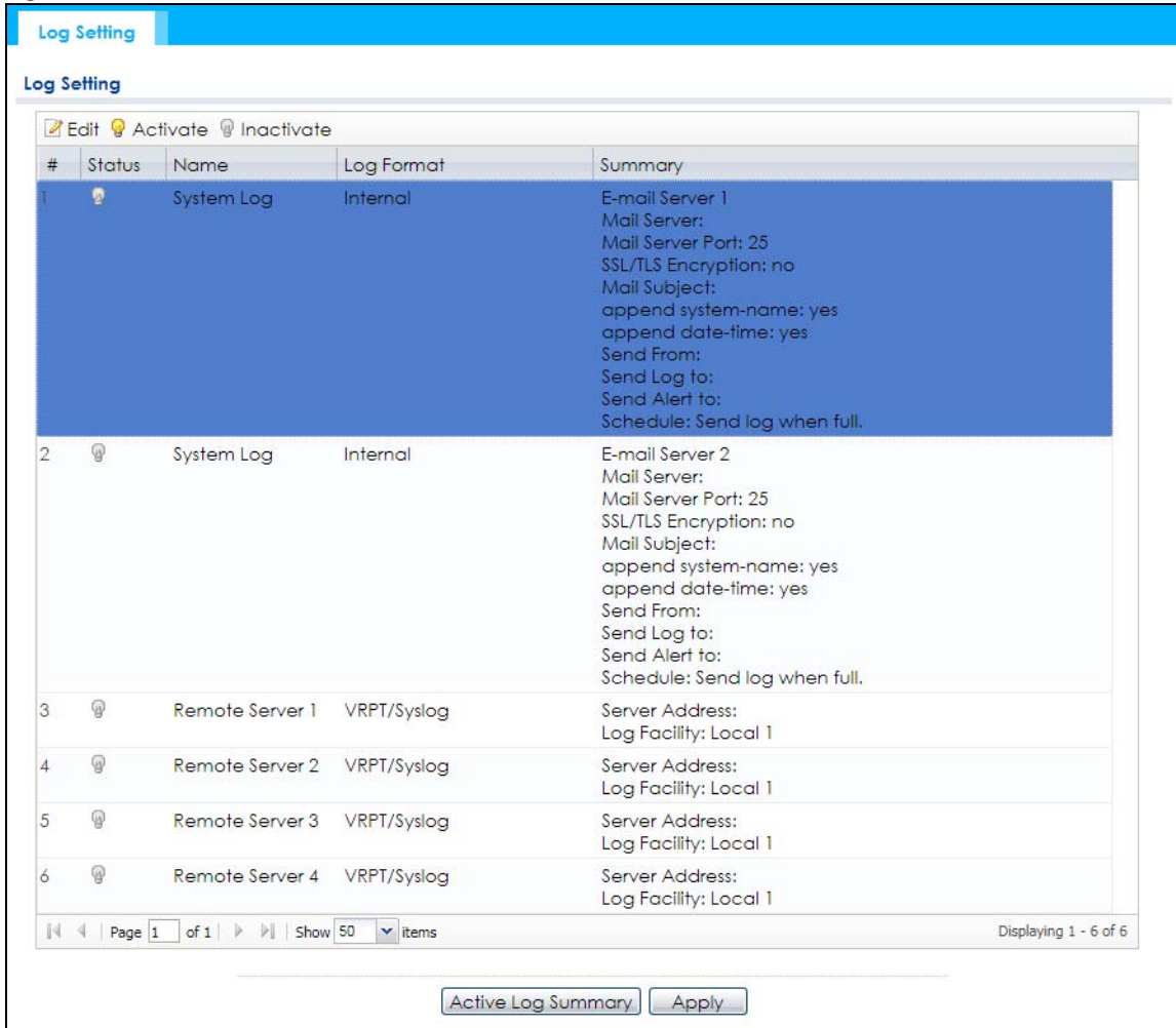
Figure 129 Configuration > Log & Report > Log Setting
