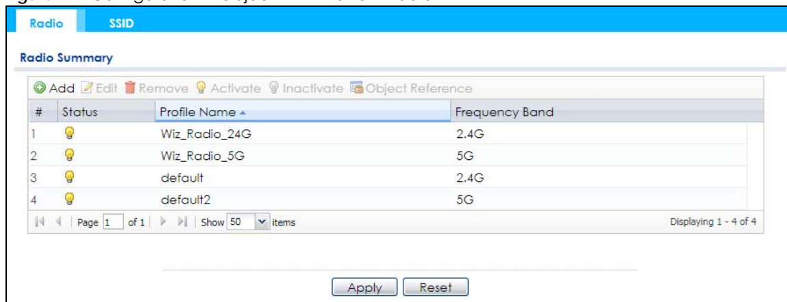
Figure 79 Configuration &gt; Object &gt; AP Profile &gt; Radio
