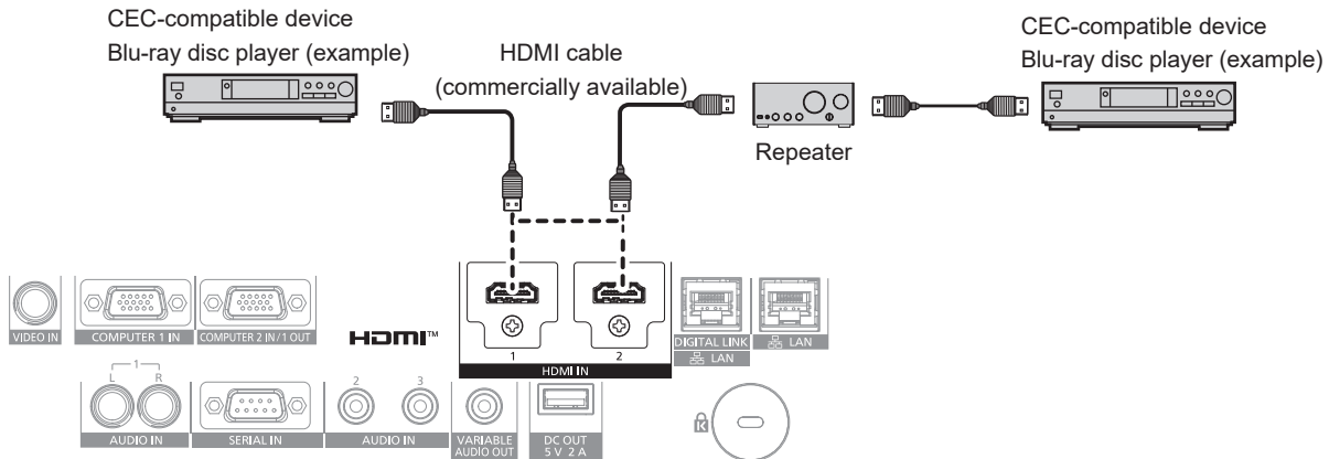
Connection example with CEC-compatible device
