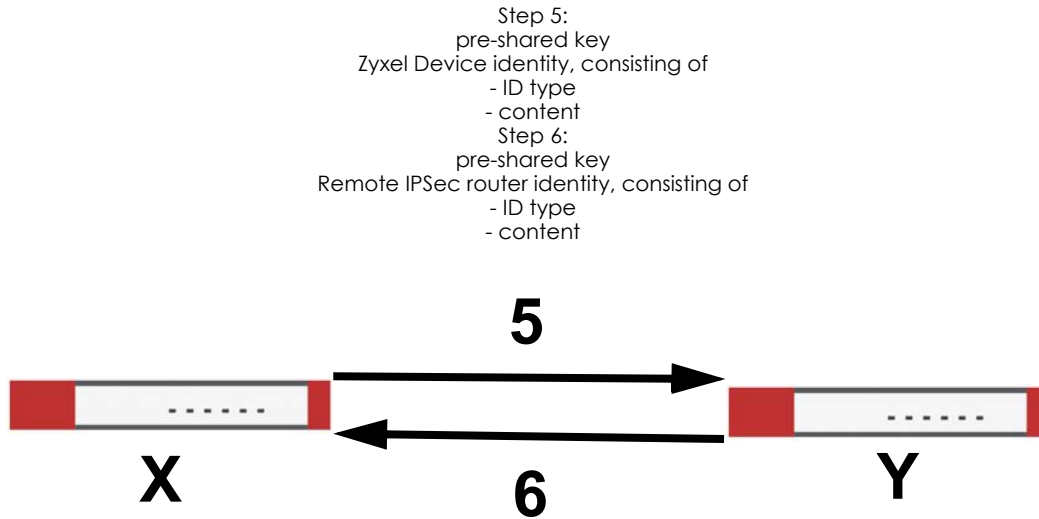
Figure 378 IKE SA: Main Negotiation Mode, Steps 5 - 6: Authentication (continued)
