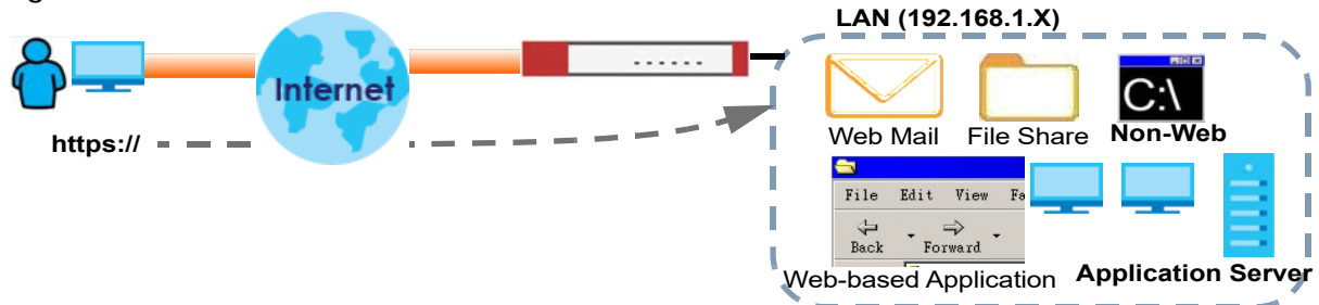
Figure 365 SSL VPN
