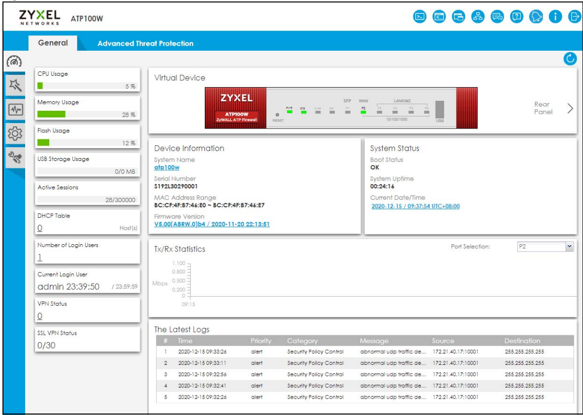
Figure 136 Dashboard ATP
