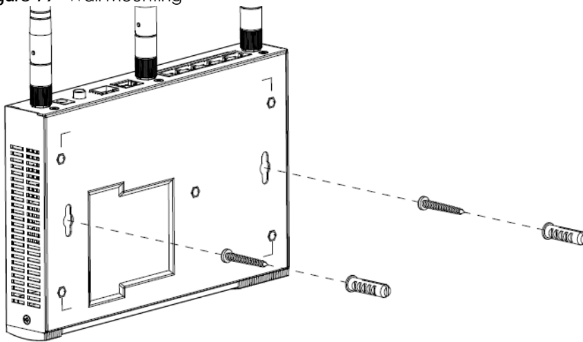
Figure 79 Wall Mounting
