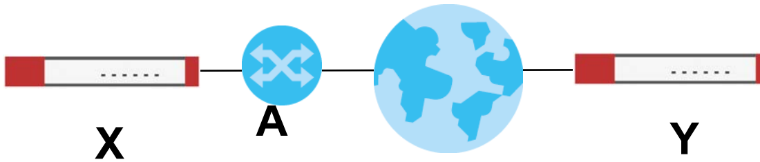
Figure 379 VPN/NAT Example
