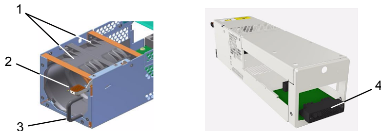
Figure 2-23 Veritas 5U84 Storage Shelf cooling module components
