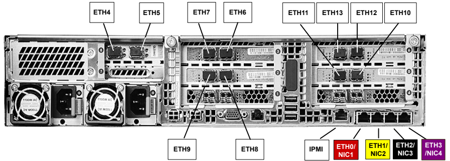
Figure 1-11 Flex &aModel; Appliance compute node NIC port assignments
