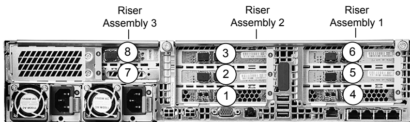
Figure 1-9 NetBackup 5340 Appliance rear panel riser assembly locations and PCIe slot number assignments
