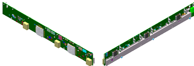
Figure 2-7 Inside and outside views of a right side Sideplane card
