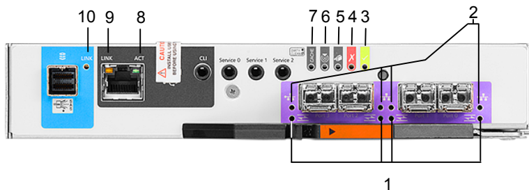
Figure 2-18 Veritas 5U84 Primary Storage Shelf Fibre Channel RAID Controller indicator LED details
