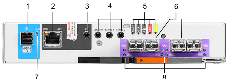
Figure 2-17 Veritas 5U84 Primary Storage Shelf Fibre Channel RAID Controller components and locations
