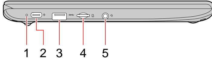
Figure 3. Lenovo 100e/300e/500e Chromebook 2nd Gen — left view
