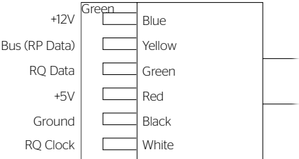
Standard RJ-25 can be used in place of RJ-14 cable
