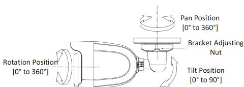
Figure 6, 3-Axis Adjustment
