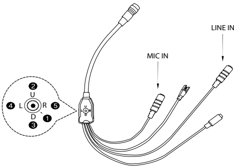
I/O Cable for CV420-CS
