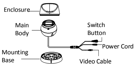
Figure 1-5 Overview of Type V Camera
