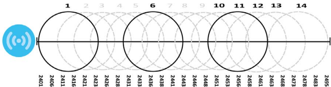
Figure 55 An Example Three-Channel Deployment
