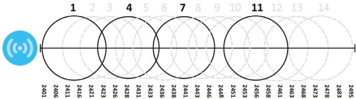
Figure 56 An Example Four-Channel Deployment
