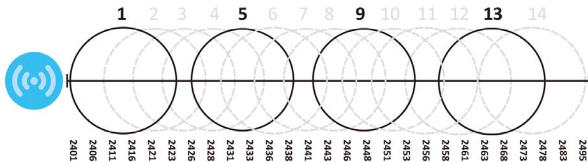
Figure 57 An Alternative Four-Channel Deployment
