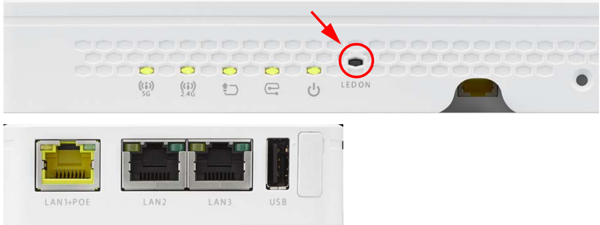
Figure 8 NWA1302-AC LEDs
