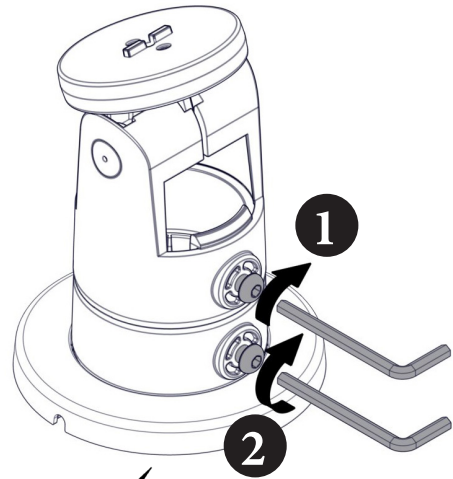
Mounting tilting module and length adapter
