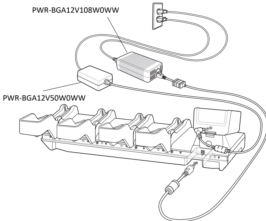
Figure 100 Power Setup with Optional Charger
