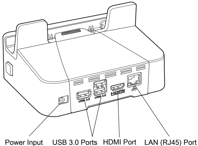
Figure 94 Rugged Communication and Charging Cradle - Rear View
