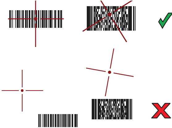
Figure 65 RS507/RS507X Pick List Mode with Multiple Barcodes in Aiming Pattern
