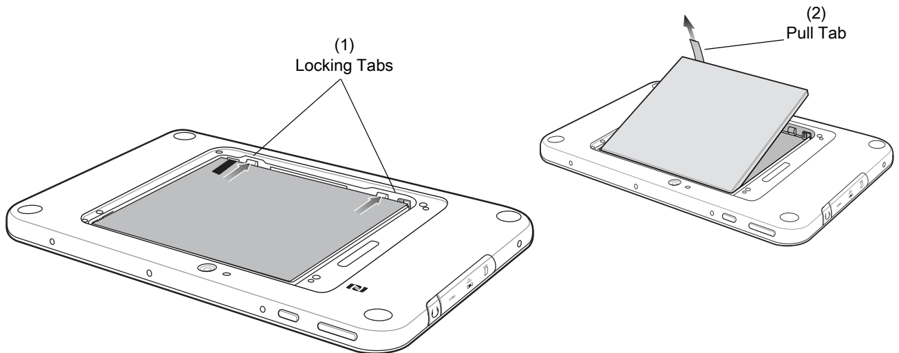
Figure 5 Removing the Battery - 8.4"
