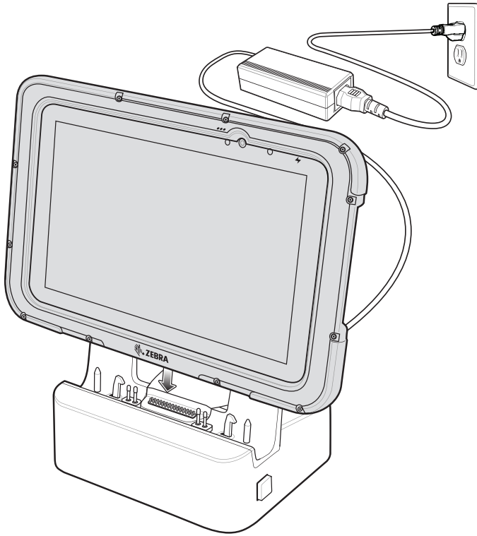
Figure 96 Insert Rugged Frame device and IO Adapter into Rugged Communication and Charging Cradle
