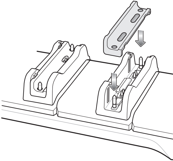
Figure 99 Install Insert in Slot
