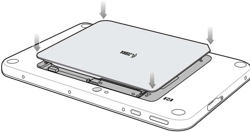
Figure 10 Aligning the Battery Cover
