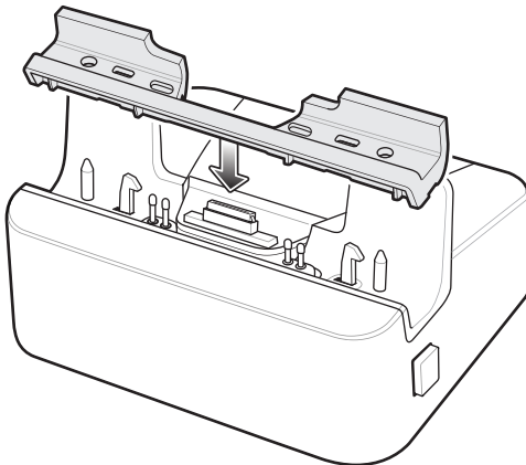
Figure 90 Align Insert with Cradle
