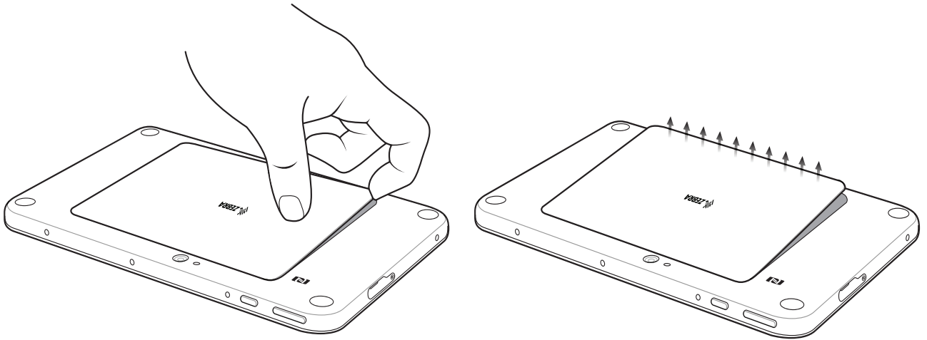
Figure 4 Lifting Battery Cover
