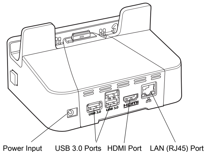
Figure 88 Communication and Charging Cradle - Rear View
