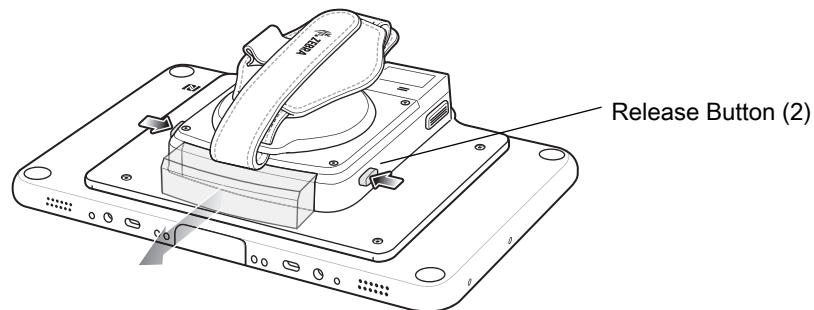
Figure 107 Remove Dummy Battery Insert
